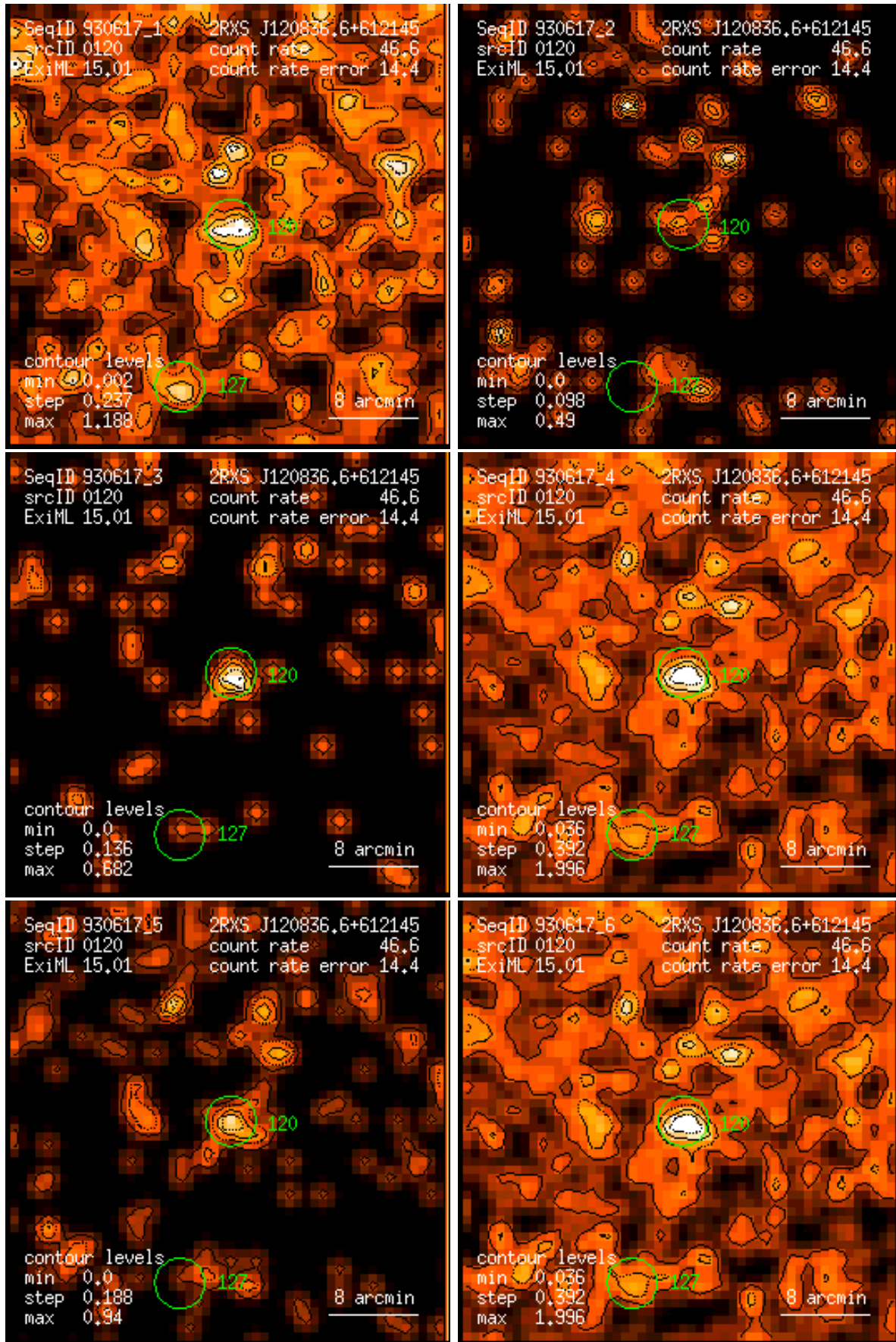
Figure 120: RASS 930617: detection 0120: band rate images, Gaussian filter: (1) PSPC channels 11 – 41, (2) 52 – 90, (3) 91 – 201, (4) 11 – 235, (5) 52 – 201, (6) 11 – 201. Broad band rates in counts/ks. Band rate contour levels in counts/ks/arcmin 2 .
