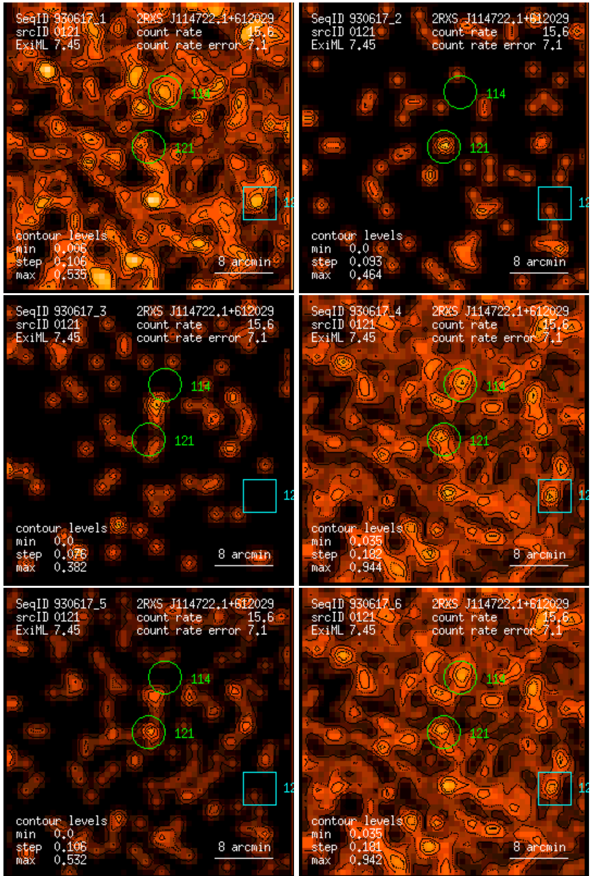
Figure 121: RASS 930617: detection 0121: band rate images, Gaussian filter: (1) PSPC channels 11 – 41, (2) 52 – 90, (3) 91 – 201, (4) 11 – 235, (5) 52 – 201, (6) 11 – 201. Broad band rates in counts/ks. Band rate contour levels in counts/ks/arcmin 2 .
