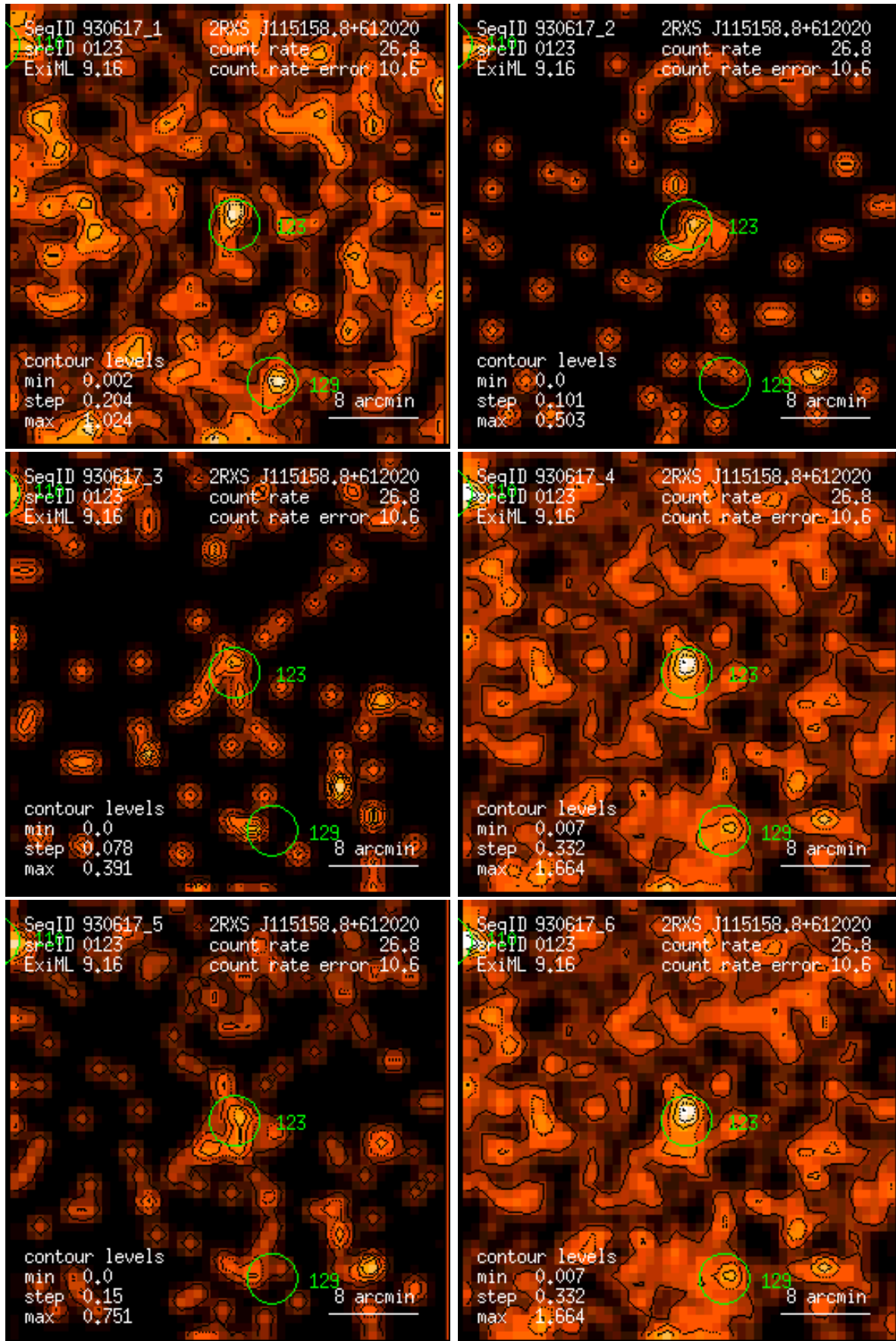
Figure 123: RASS 930617: detection 0123: band rate images, Gaussian filter: (1) PSPC channels 11 – 41, (2) 52 – 90, (3) 91 – 201, (4) 11 – 235, (5) 52 – 201, (6) 11 – 201. Broad band rates in counts/ks. Band rate contour levels in counts/ks/arcmin 2 .
