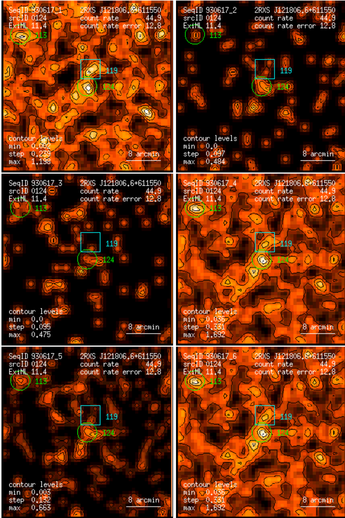
Figure 124: RASS 930617: detection 0124: band rate images, Gaussian filter: (1) PSPC channels 11 – 41, (2) 52 – 90, (3) 91 – 201, (4) 11 – 235, (5) 52 – 201, (6) 11 – 201. Broad band rates in counts/ks. Band rate contour levels in counts/ks/arcmin 2 .
