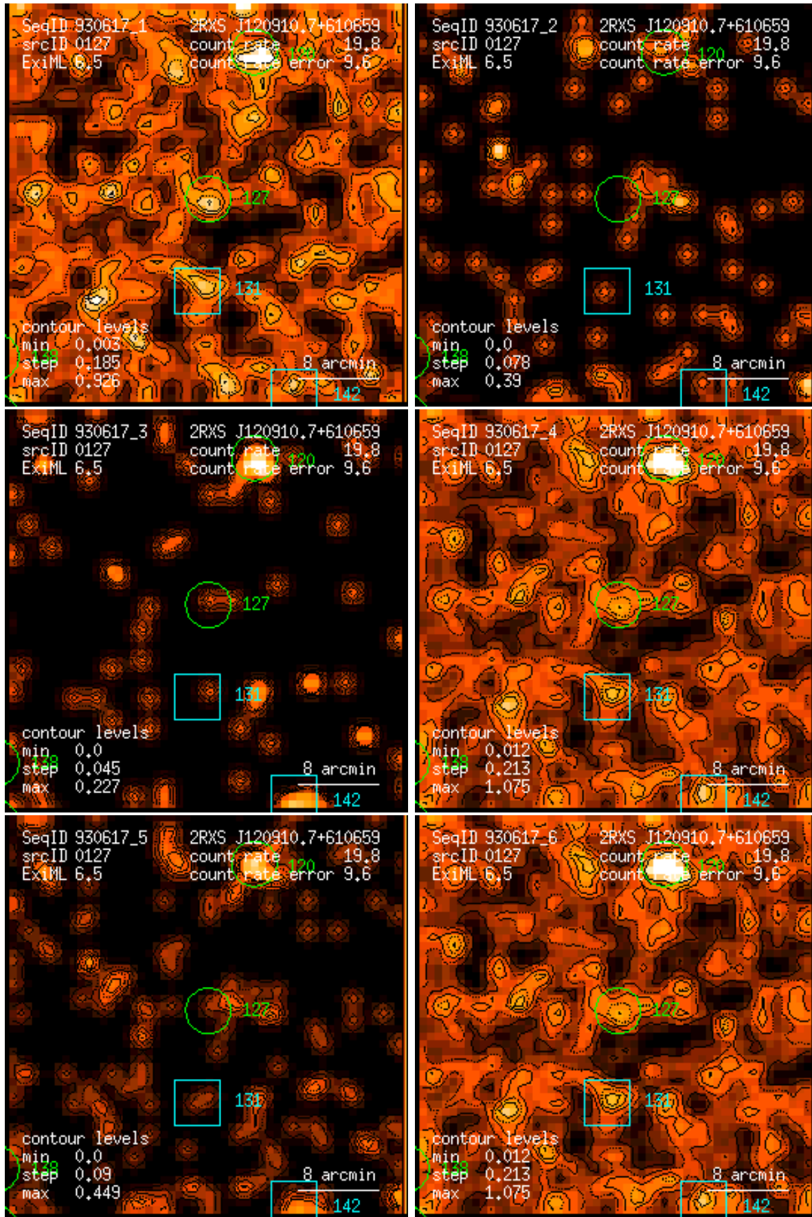
Figure 127: RASS 930617: detection 0127: band rate images, Gaussian filter: (1) PSPC channels 11 – 41, (2) 52 – 90, (3) 91 – 201, (4) 11 – 235, (5) 52 – 201, (6) 11 – 201. Broad band rates in counts/ks. Band rate contour levels in counts/ks/arcmin 2 .
