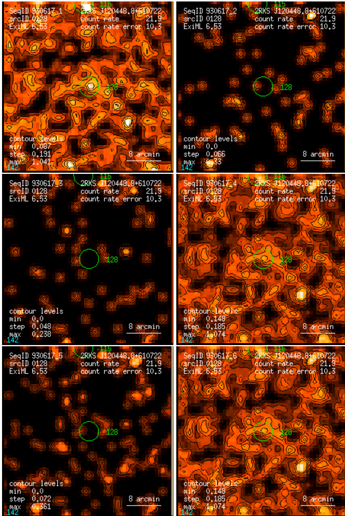
Figure 128: RASS 930617: detection 0128: band rate images, Gaussian filter: (1) PSPC channels 11 – 41, (2) 52 – 90, (3) 91 – 201, (4) 11 – 235, (5) 52 – 201, (6) 11 – 201. Broad band rates in counts/ks. Band rate contour levels in counts/ks/arcmin 2 .
