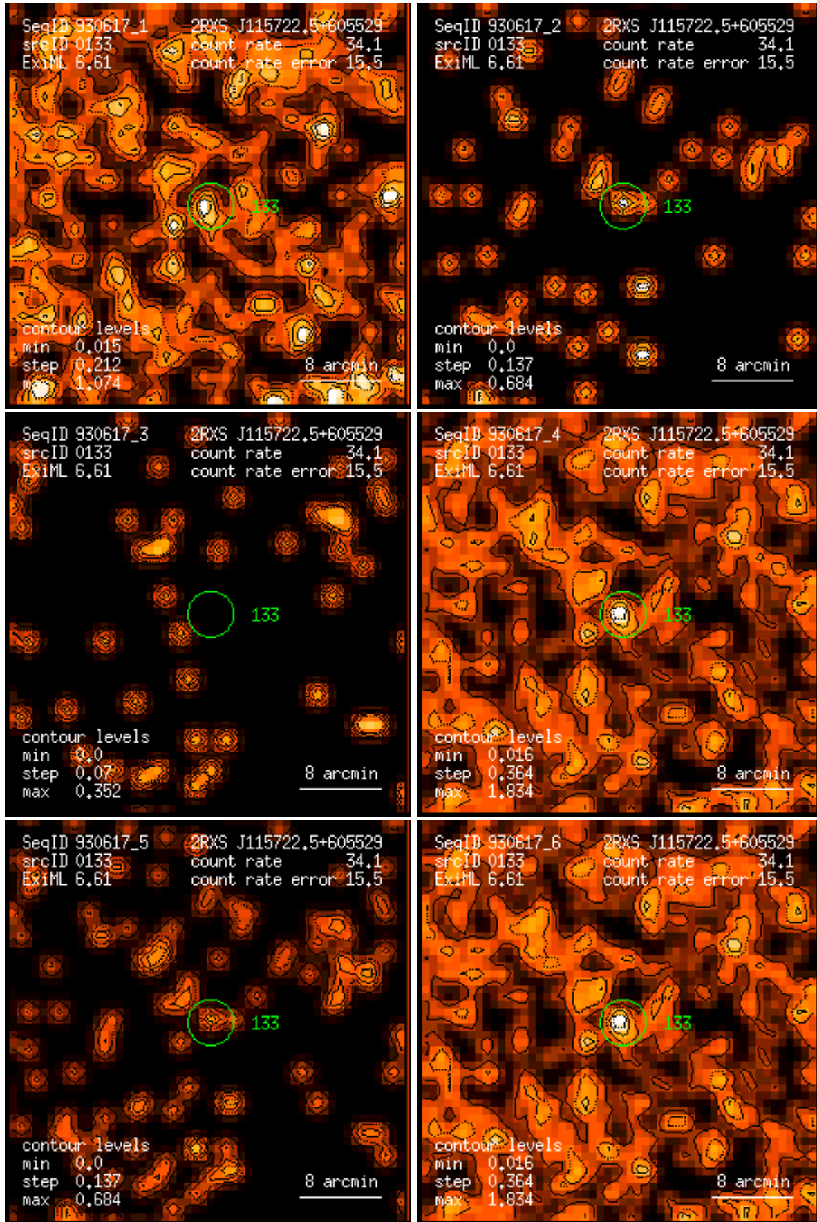
Figure 133: RASS 930617: detection 0133: band rate images, Gaussian filter: (1) PSPC channels 11 – 41, (2) 52 – 90, (3) 91 – 201, (4) 11 – 235, (5) 52 – 201, (6) 11 – 201. Broad band rates in counts/ks. Band rate contour levels in counts/ks/arcmin 2 .
