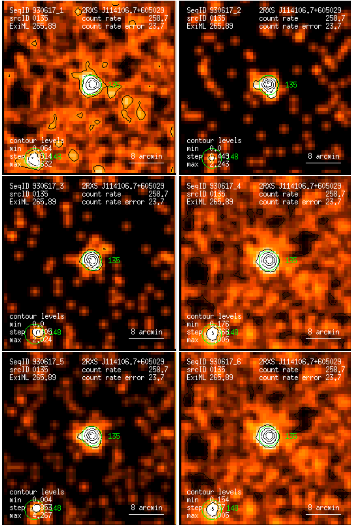
Figure 135: RASS 930617: detection 0135: band rate images, Gaussian filter: (1) PSPC channels 11 – 41, (2) 52 – 90, (3) 91 – 201, (4) 11 – 235, (5) 52 – 201, (6) 11 – 201. Broad band rates in counts/ks. Band rate contour levels in counts/ks/arcmin 2 .
