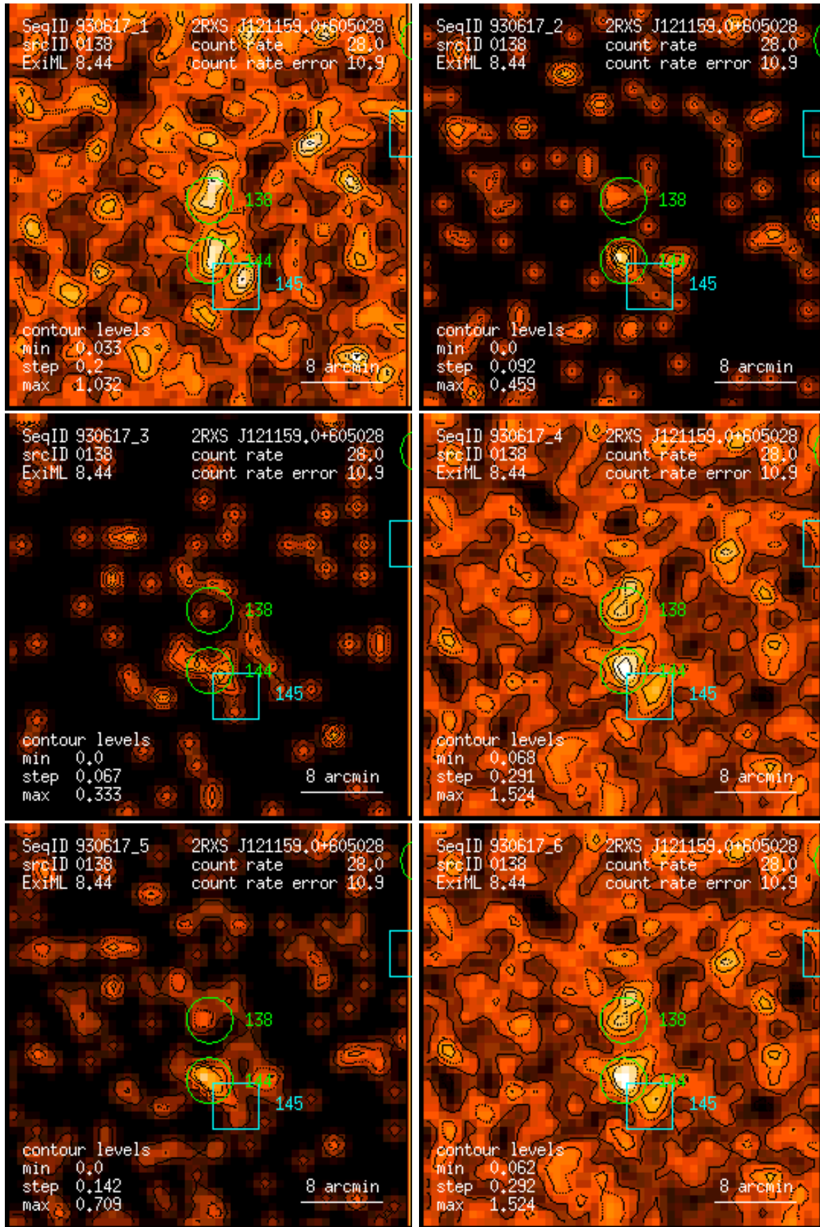
Figure 138: RASS 930617: detection 0138: band rate images, Gaussian filter: (1) PSPC channels 11 – 41, (2) 52 – 90, (3) 91 – 201, (4) 11 – 235, (5) 52 – 201, (6) 11 – 201. Broad band rates in counts/ks. Band rate contour levels in counts/ks/arcmin 2 .
