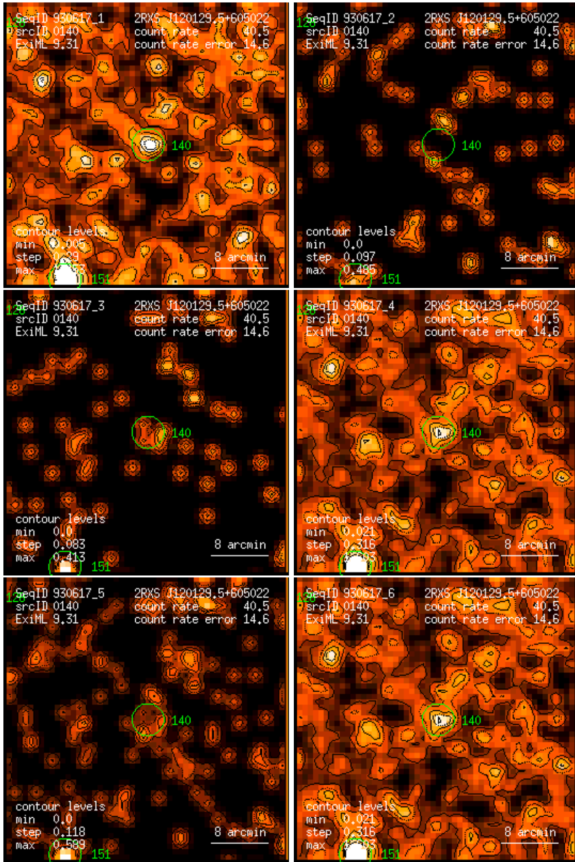
Figure 140: RASS 930617: detection 0140: band rate images, Gaussian filter: (1) PSPC channels 11 – 41, (2) 52 – 90, (3) 91 – 201, (4) 11 – 235, (5) 52 – 201, (6) 11 – 201. Broad band rates in counts/ks. Band rate contour levels in counts/ks/arcmin 2 .
