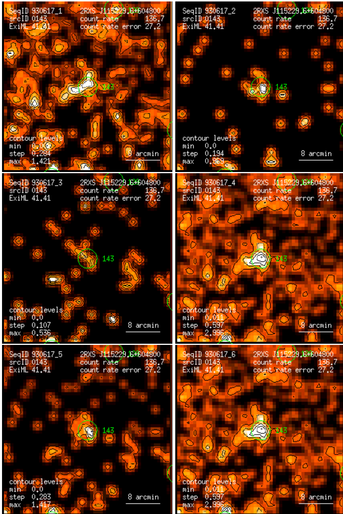
Figure 143: RASS 930617: detection 0143: band rate images, Gaussian filter: (1) PSPC channels 11 – 41, (2) 52 – 90, (3) 91 – 201, (4) 11 – 235, (5) 52 – 201, (6) 11 – 201. Broad band rates in counts/ks. Band rate contour levels in counts/ks/arcmin 2 .
