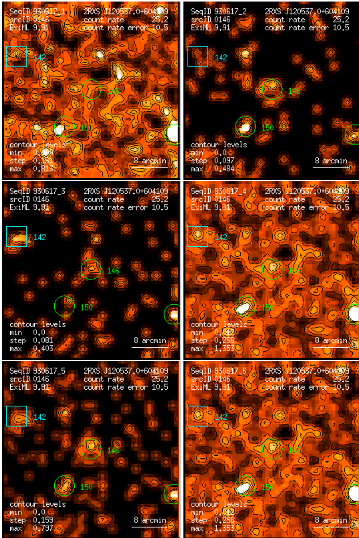
Figure 146: RASS 930617: detection 0146: band rate images, Gaussian filter: (1) PSPC channels 11 – 41, (2) 52 – 90, (3) 91 – 201, (4) 11 – 235, (5) 52 – 201, (6) 11 – 201. Broad band rates in counts/ks. Band rate contour levels in counts/ks/arcmin 2 .
