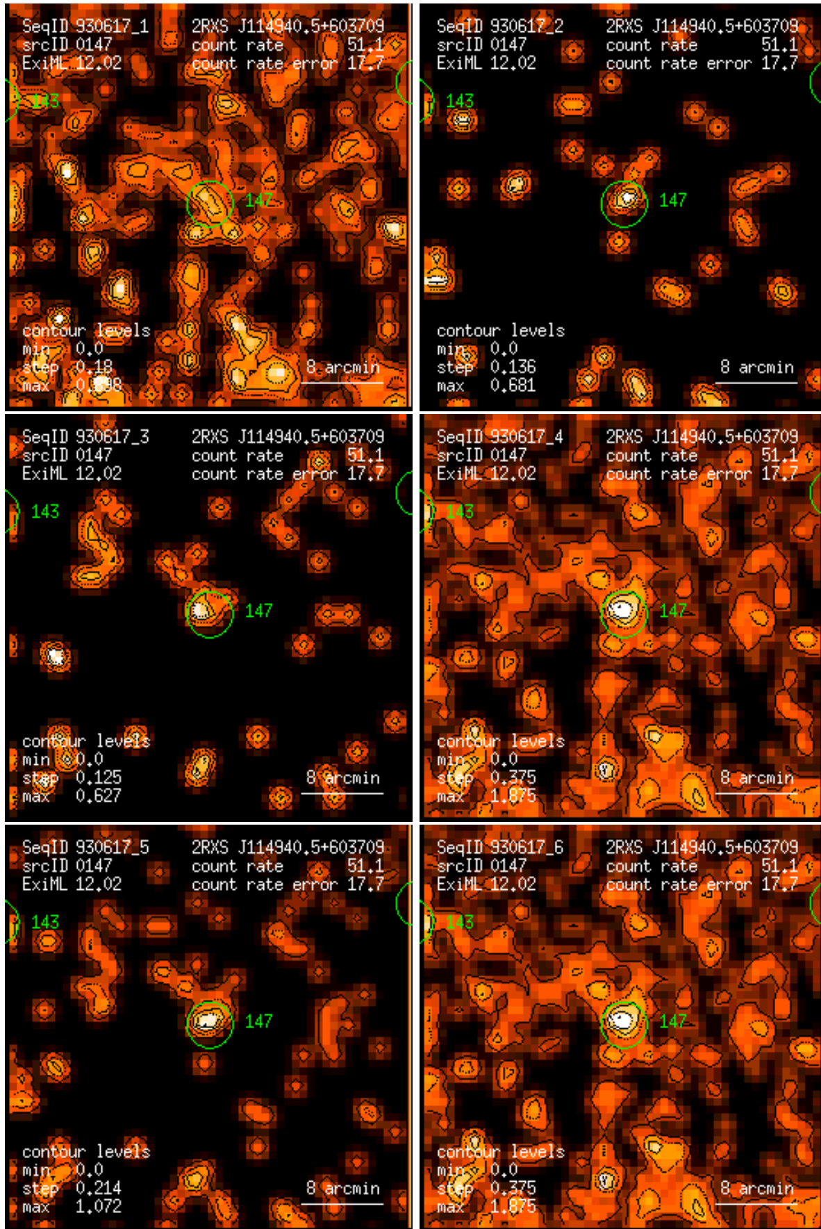
Figure 147: RASS 930617: detection 0147: band rate images, Gaussian filter: (1) PSPC channels 11 – 41, (2) 52 – 90, (3) 91 – 201, (4) 11 – 235, (5) 52 – 201, (6) 11 – 201. Broad band rates in counts/ks. Band rate contour levels in counts/ks/arcmin 2 .
