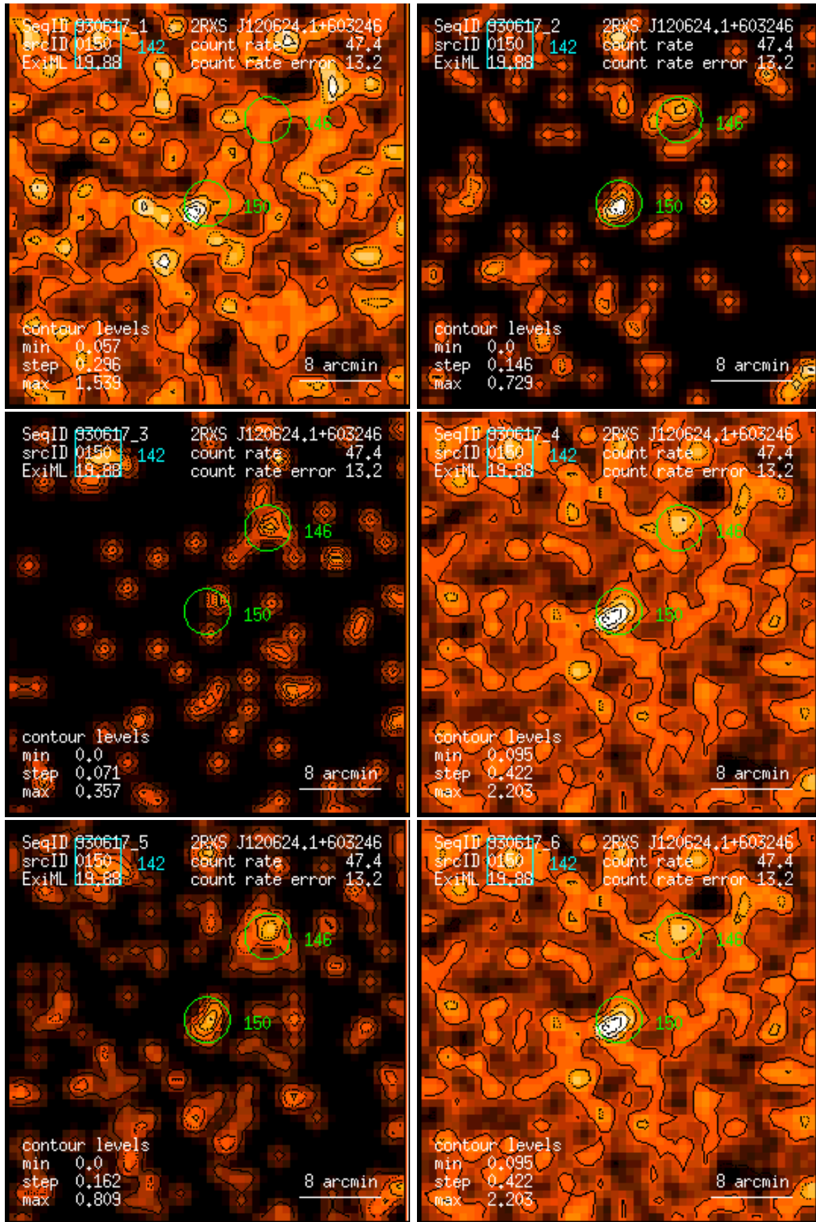
Figure 150: RASS 930617: detection 0150: band rate images, Gaussian filter: (1) PSPC channels 11 – 41, (2) 52 – 90, (3) 91 – 201, (4) 11 – 235, (5) 52 – 201, (6) 11 – 201. Broad band rates in counts/ks. Band rate contour levels in counts/ks/arcmin 2 .
