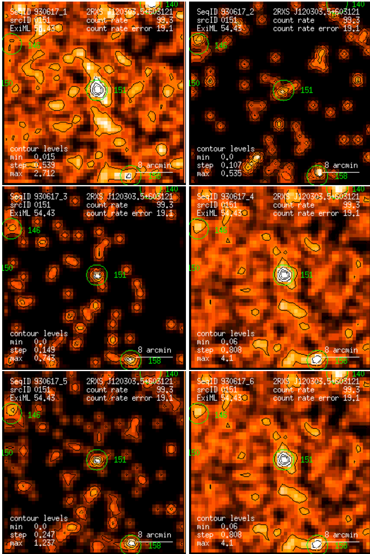
Figure 151: RASS 930617: detection 0151: band rate images, Gaussian filter: (1) PSPC channels 11 – 41, (2) 52 – 90, (3) 91 – 201, (4) 11 – 235, (5) 52 – 201, (6) 11 – 201. Broad band rates in counts/ks. Band rate contour levels in counts/ks/arcmin 2 .
