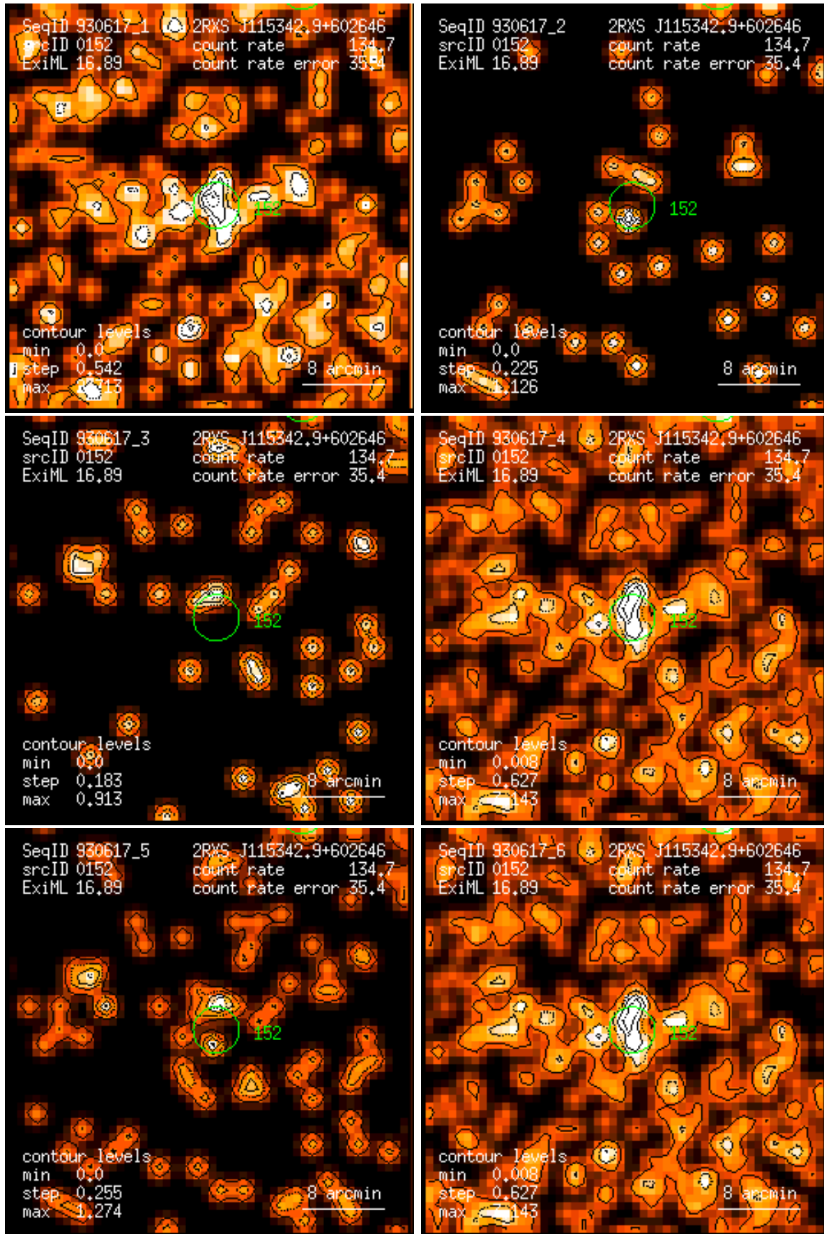
Figure 152: RASS 930617: detection 0152: band rate images, Gaussian filter: (1) PSPC channels 11 – 41, (2) 52 – 90, (3) 91 – 201, (4) 11 – 235, (5) 52 – 201, (6) 11 – 201. Broad band rates in counts/ks. Band rate contour levels in counts/ks/arcmin 2 .
