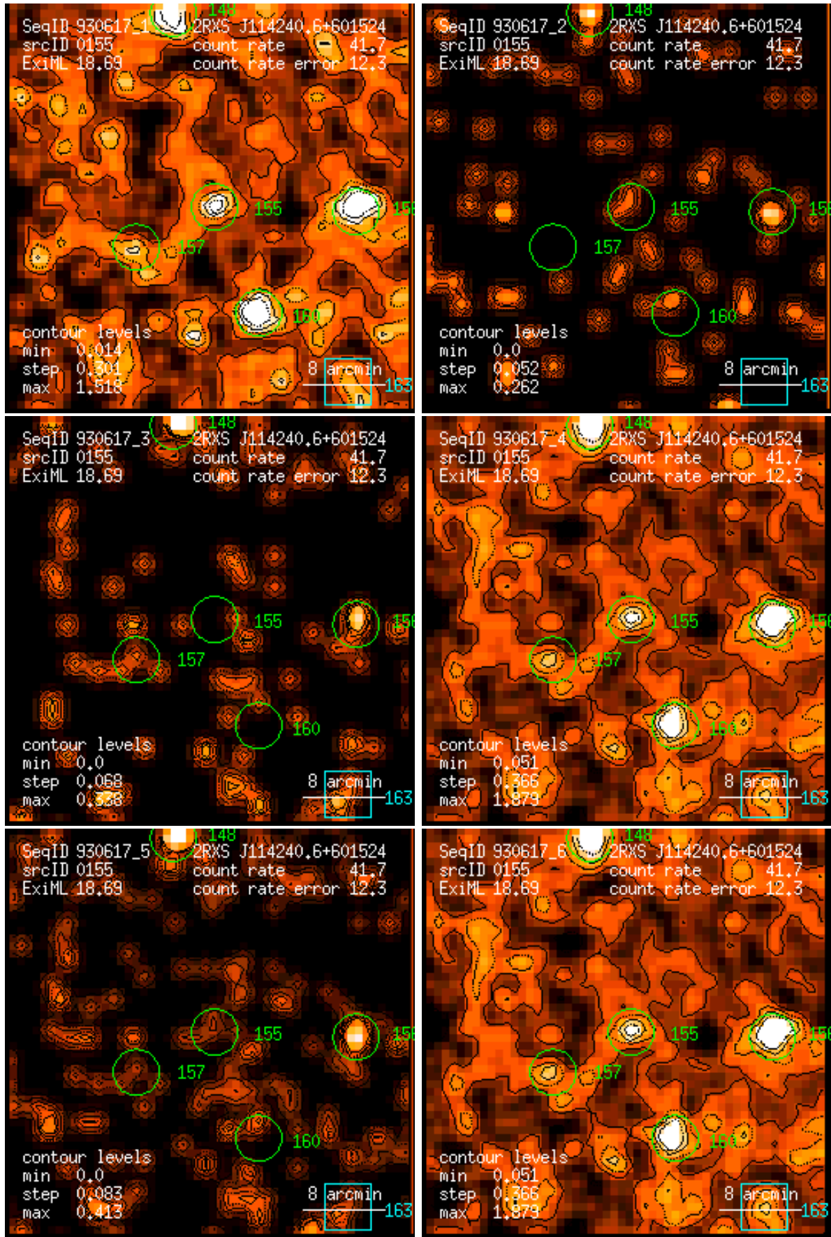
Figure 155: RASS 930617: detection 0155: band rate images, Gaussian filter: (1) PSPC channels 11 – 41, (2) 52 – 90, (3) 91 – 201, (4) 11 – 235, (5) 52 – 201, (6) 11 – 201. Broad band rates in counts/ks. Band rate contour levels in counts/ks/arcmin 2 .
