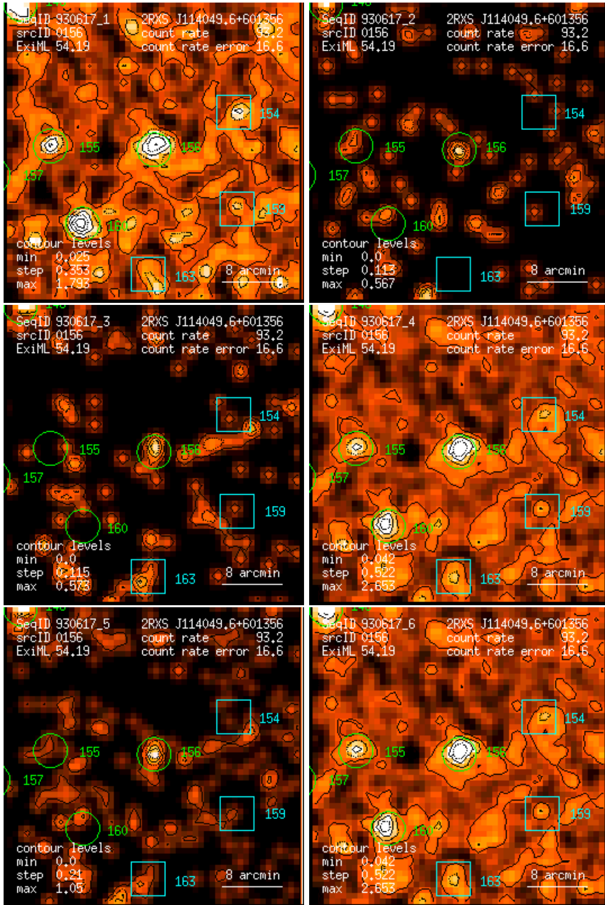
Figure 156: RASS 930617: detection 0156: band rate images, Gaussian filter: (1) PSPC channels 11 – 41, (2) 52 – 90, (3) 91 – 201, (4) 11 – 235, (5) 52 – 201, (6) 11 – 201. Broad band rates in counts/ks. Band rate contour levels in counts/ks/arcmin 2 .
