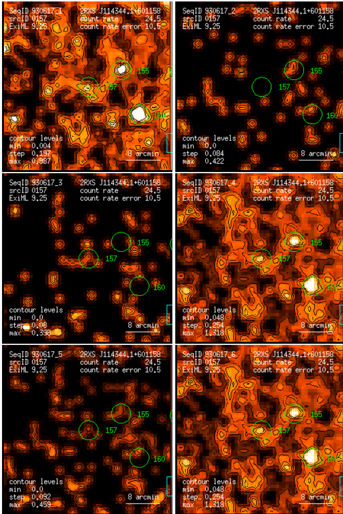
Figure 157: RASS 930617: detection 0157: band rate images, Gaussian filter: (1) PSPC channels 11 – 41, (2) 52 – 90, (3) 91 – 201, (4) 11 – 235, (5) 52 – 201, (6) 11 – 201. Broad band rates in counts/ks. Band rate contour levels in counts/ks/arcmin 2 .
