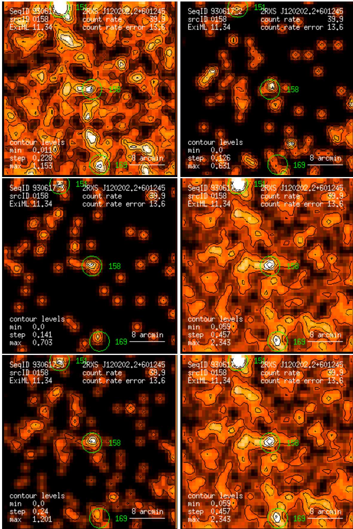
Figure 158: RASS 930617: detection 0158: band rate images, Gaussian filter: (1) PSPC channels 11 – 41, (2) 52 – 90, (3) 91 – 201, (4) 11 – 235, (5) 52 – 201, (6) 11 – 201. Broad band rates in counts/ks. Band rate contour levels in counts/ks/arcmin 2 .
