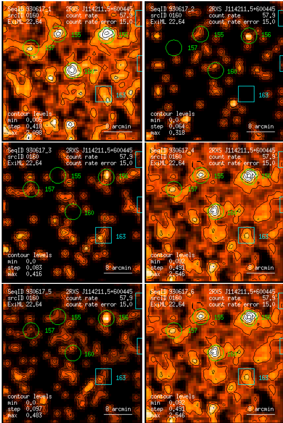
Figure 160: RASS 930617: detection 0160: band rate images, Gaussian filter: (1) PSPC channels 11 – 41, (2) 52 – 90, (3) 91 – 201, (4) 11 – 235, (5) 52 – 201, (6) 11 – 201. Broad band rates in counts/ks. Band rate contour levels in counts/ks/arcmin 2 .
