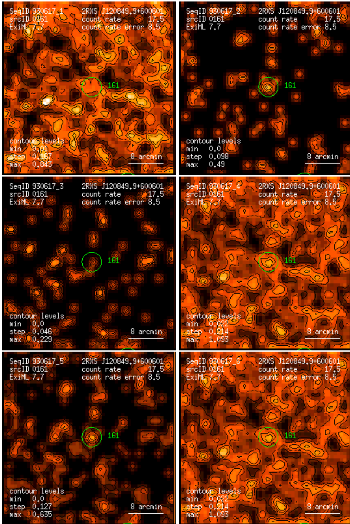
Figure 161: RASS 930617: detection 0161: band rate images, Gaussian filter: (1) PSPC channels 11 – 41, (2) 52 – 90, (3) 91 – 201, (4) 11 – 235, (5) 52 – 201, (6) 11 – 201. Broad band rates in counts/ks. Band rate contour levels in counts/ks/arcmin 2 .
