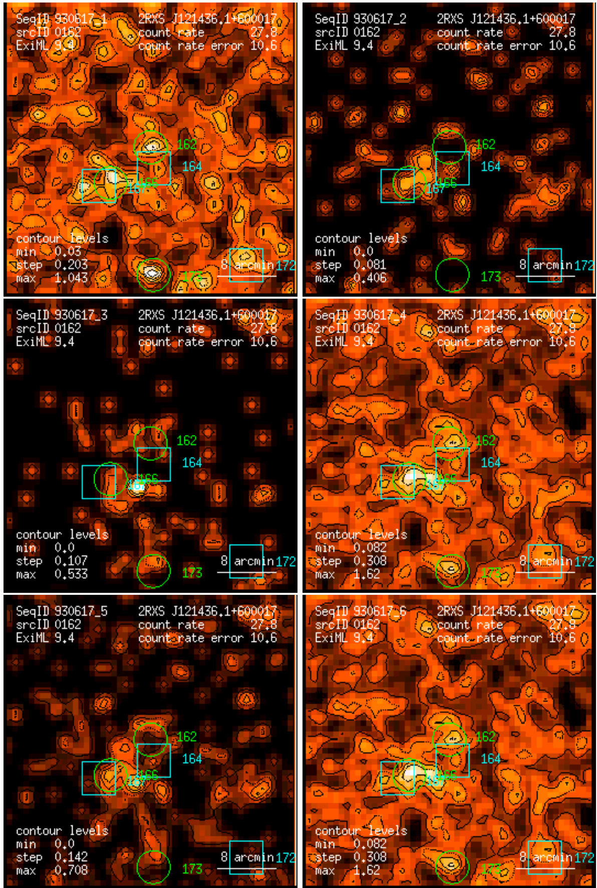
Figure 162: RASS 930617: detection 0162: band rate images, Gaussian filter: (1) PSPC channels 11 – 41, (2) 52 – 90, (3) 91 – 201, (4) 11 – 235, (5) 52 – 201, (6) 11 – 201. Broad band rates in counts/ks. Band rate contour levels in counts/ks/arcmin 2 .
