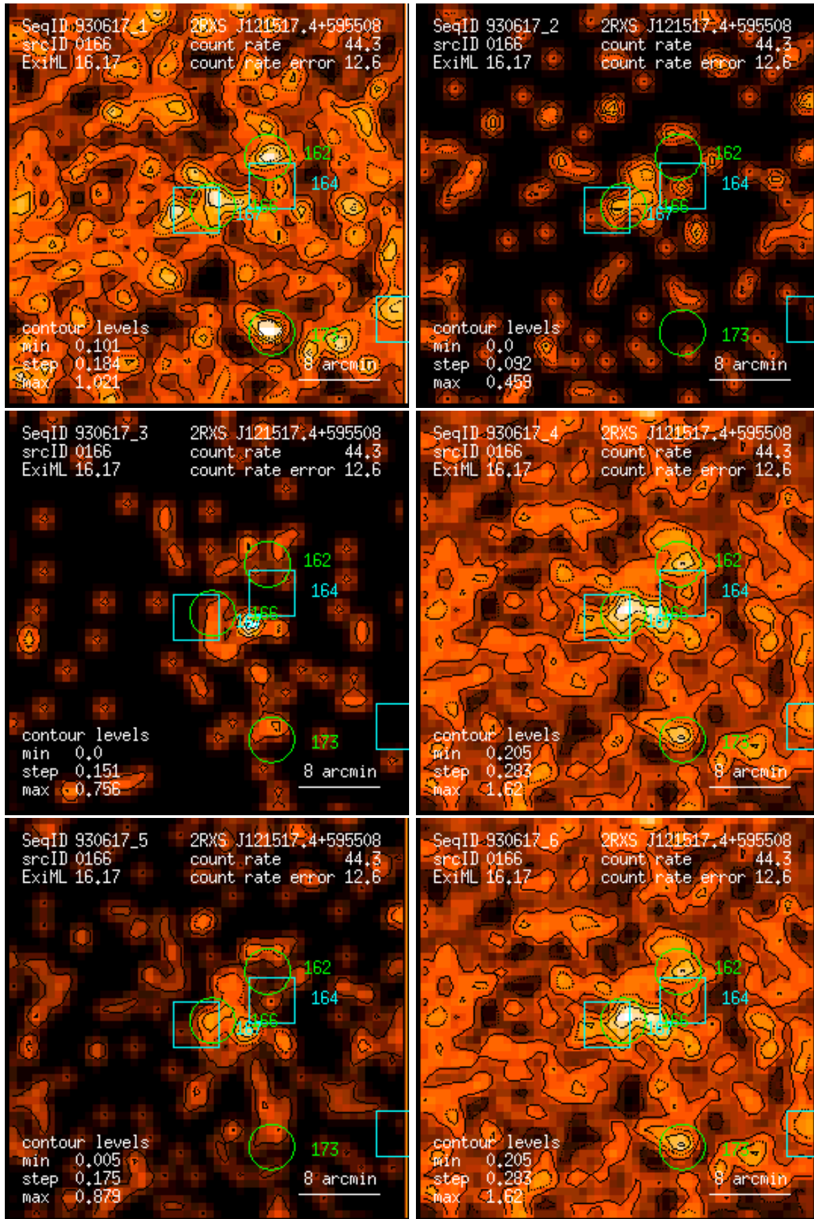
Figure 166: RASS 930617: detection 0166: band rate images, Gaussian filter: (1) PSPC channels 11 – 41, (2) 52 – 90, (3) 91 – 201, (4) 11 – 235, (5) 52 – 201, (6) 11 – 201. Broad band rates in counts/ks. Band rate contour levels in counts/ks/arcmin 2 .
