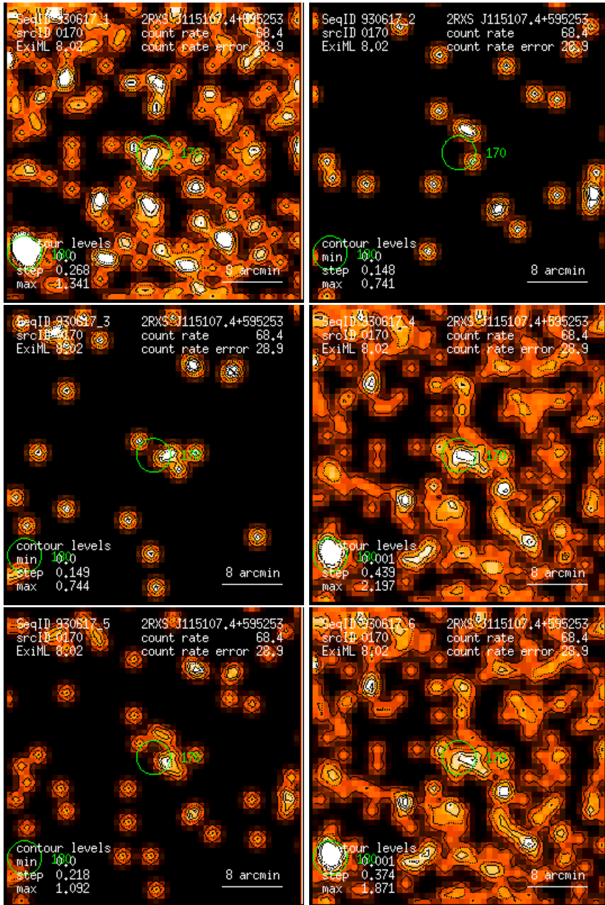
Figure 170: RASS 930617: detection 0170: band rate images, Gaussian filter: (1) PSPC channels 11 – 41, (2) 52 – 90, (3) 91 – 201, (4) 11 – 235, (5) 52 – 201, (6) 11 – 201. Broad band rates in counts/ks. Band rate contour levels in counts/ks/arcmin 2 .
