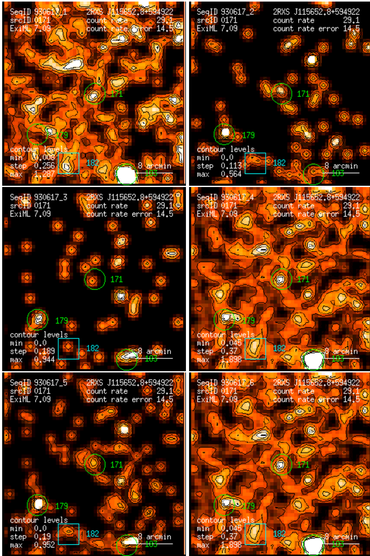
Figure 171: RASS 930617: detection 0171: band rate images, Gaussian filter: (1) PSPC channels 11 – 41, (2) 52 – 90, (3) 91 – 201, (4) 11 – 235, (5) 52 – 201, (6) 11 – 201. Broad band rates in counts/ks. Band rate contour levels in counts/ks/arcmin 2 .
