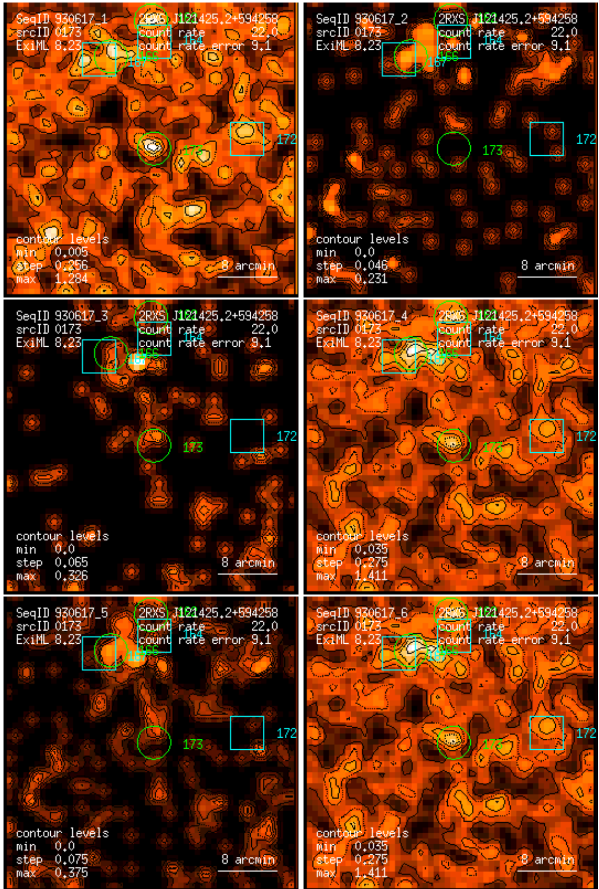
Figure 173: RASS 930617: detection 0173: band rate images, Gaussian filter: (1) PSPC channels 11 – 41, (2) 52 – 90, (3) 91 – 201, (4) 11 – 235, (5) 52 – 201, (6) 11 – 201. Broad band rates in counts/ks. Band rate contour levels in counts/ks/arcmin 2 .
