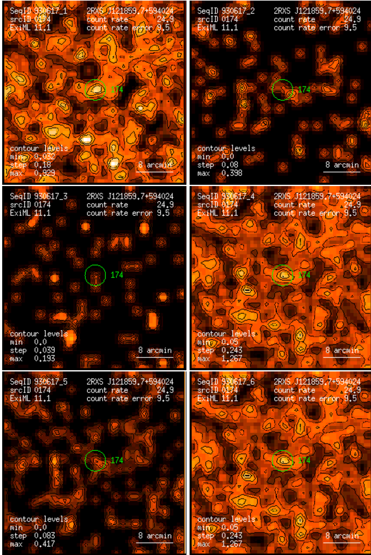
Figure 174: RASS 930617: detection 0174: band rate images, Gaussian filter: (1) PSPC channels 11 – 41, (2) 52 – 90, (3) 91 – 201, (4) 11 – 235, (5) 52 – 201, (6) 11 – 201. Broad band rates in counts/ks. Band rate contour levels in counts/ks/arcmin 2 .
