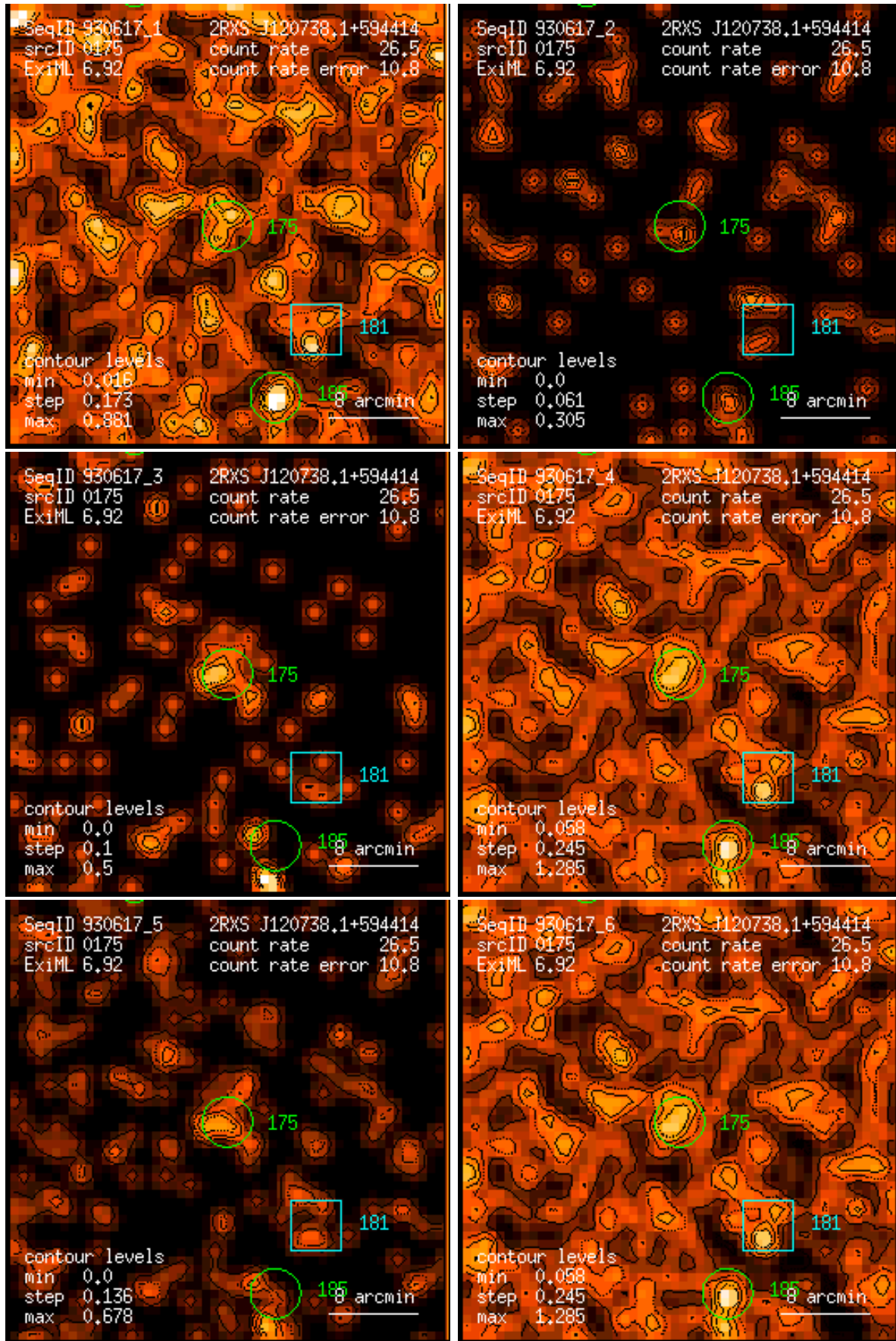
Figure 175: RASS 930617: detection 0175: band rate images, Gaussian filter: (1) PSPC channels 11 – 41, (2) 52 – 90, (3) 91 – 201, (4) 11 – 235, (5) 52 – 201, (6) 11 – 201. Broad band rates in counts/ks. Band rate contour levels in counts/ks/arcmin 2 .
