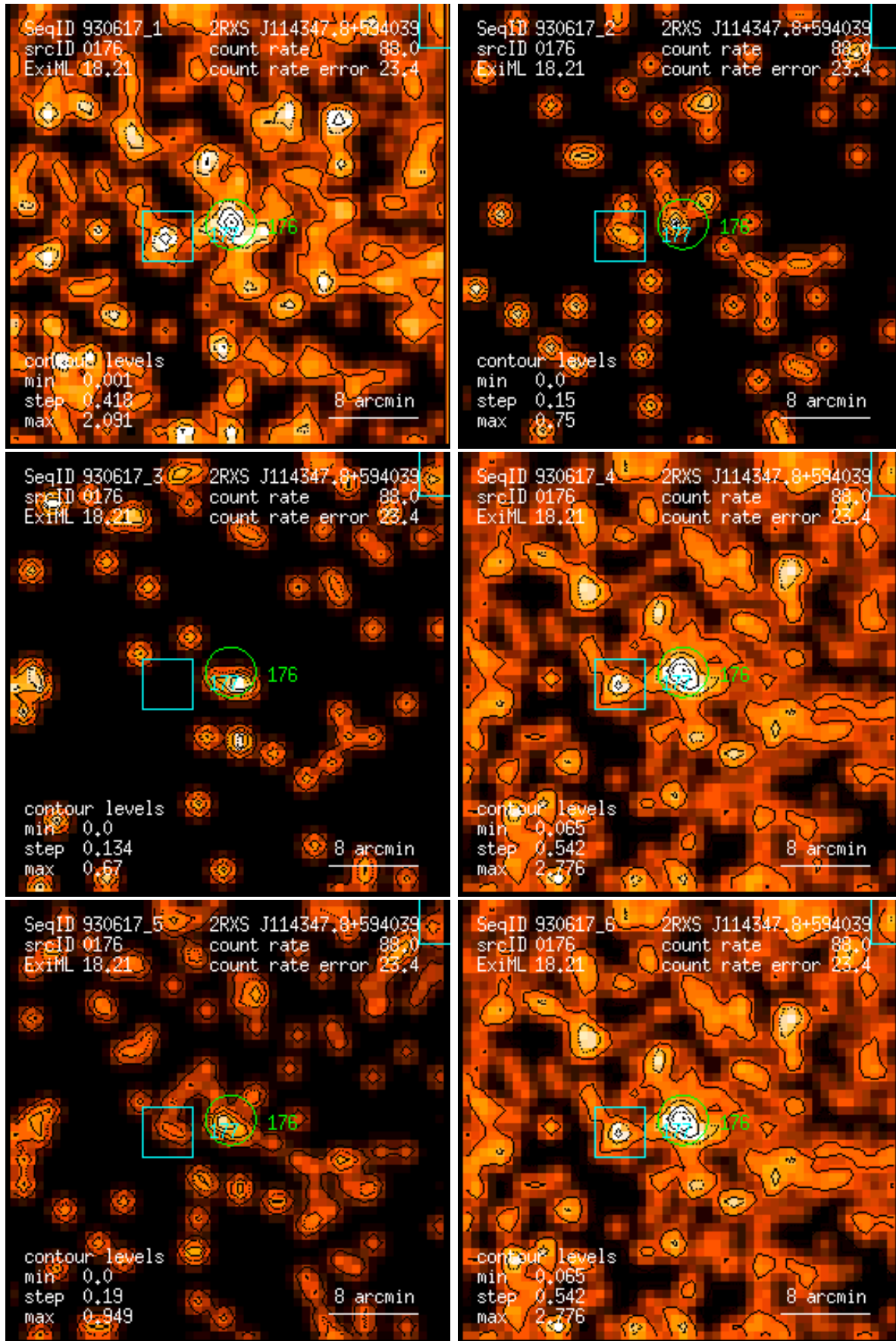
Figure 176: RASS 930617: detection 0176: band rate images, Gaussian filter: (1) PSPC channels 11 – 41, (2) 52 – 90, (3) 91 – 201, (4) 11 – 235, (5) 52 – 201, (6) 11 – 201. Broad band rates in counts/ks. Band rate contour levels in counts/ks/arcmin 2 .
