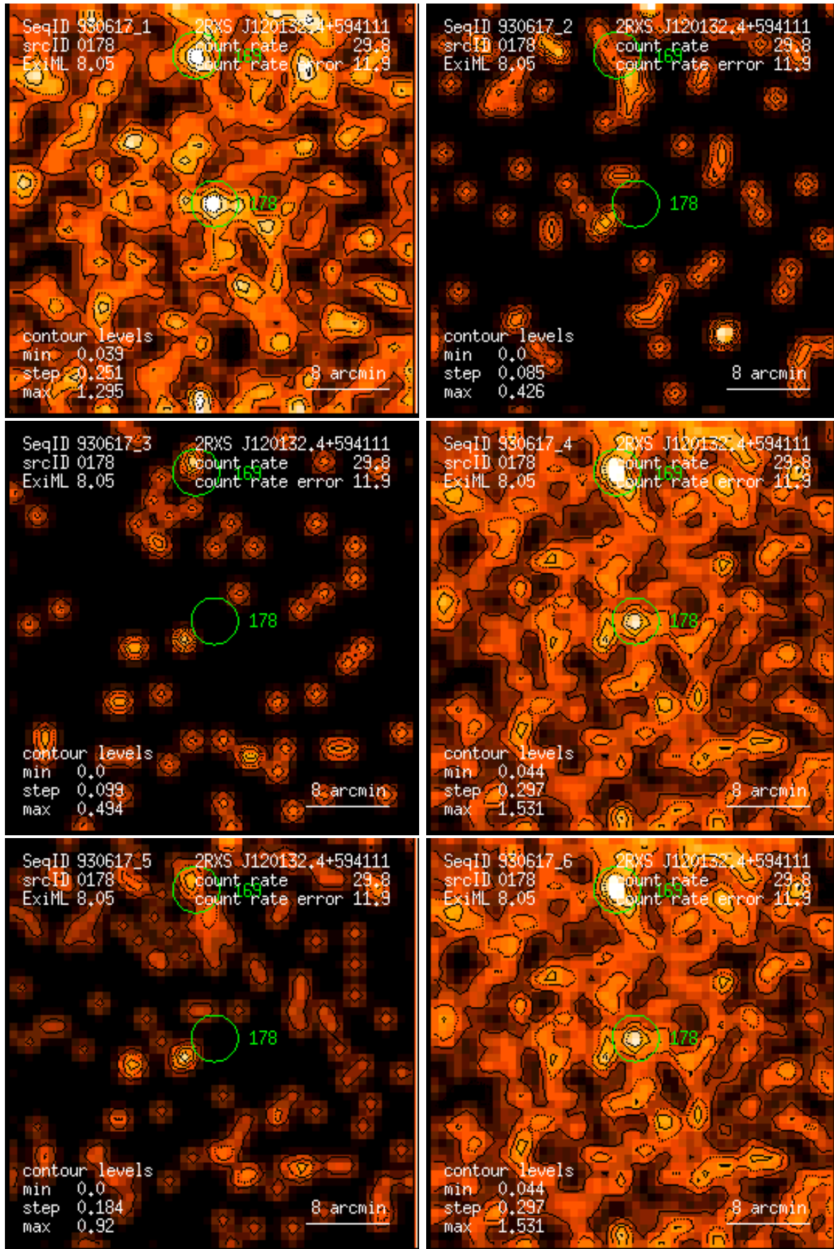
Figure 178: RASS 930617: detection 0178: band rate images, Gaussian filter: (1) PSPC channels 11 – 41, (2) 52 – 90, (3) 91 – 201, (4) 11 – 235, (5) 52 – 201, (6) 11 – 201. Broad band rates in counts/ks. Band rate contour levels in counts/ks/arcmin 2 .
