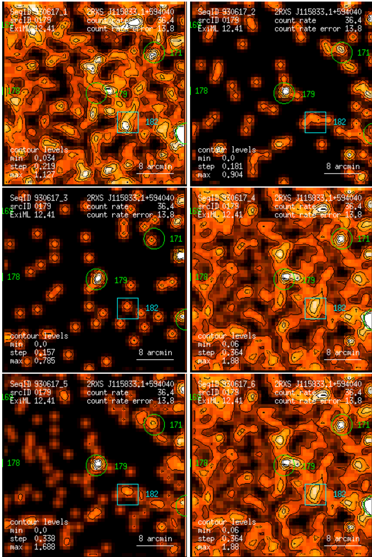
Figure 179: RASS 930617: detection 0179: band rate images, Gaussian filter: (1) PSPC channels 11 – 41, (2) 52 – 90, (3) 91 – 201, (4) 11 – 235, (5) 52 – 201, (6) 11 – 201. Broad band rates in counts/ks. Band rate contour levels in counts/ks/arcmin 2 .
