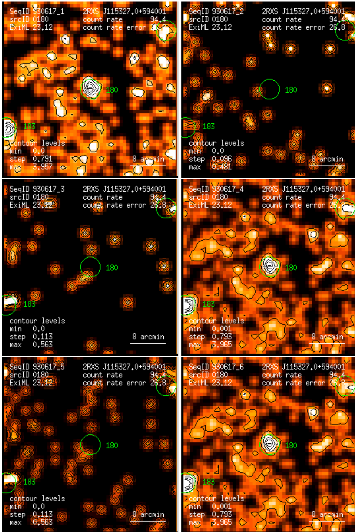
Figure 180: RASS 930617: detection 0180: band rate images, Gaussian filter: (1) PSPC channels 11 – 41, (2) 52 – 90, (3) 91 – 201, (4) 11 – 235, (5) 52 – 201, (6) 11 – 201. Broad band rates in counts/ks. Band rate contour levels in counts/ks/arcmin 2 .
