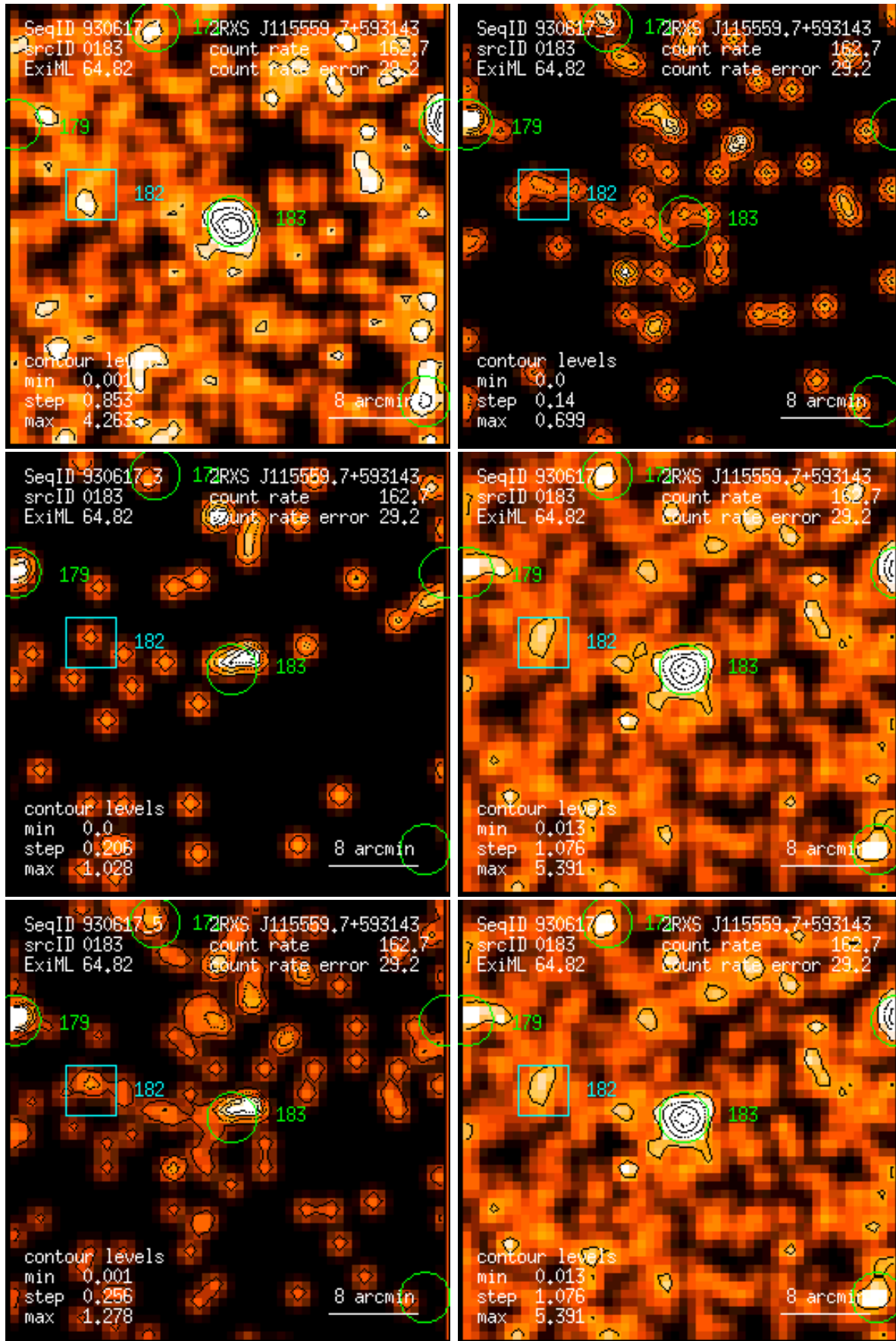
Figure 183: RASS 930617: detection 0183: band rate images, Gaussian filter: (1) PSPC channels 11 – 41, (2) 52 – 90, (3) 91 – 201, (4) 11 – 235, (5) 52 – 201, (6) 11 – 201. Broad band rates in counts/ks. Band rate contour levels in counts/ks/arcmin 2 .
