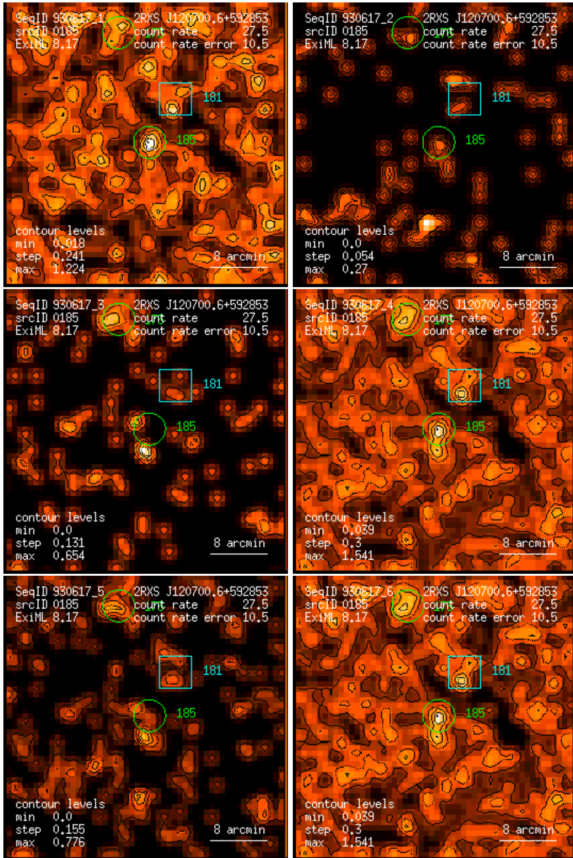
Figure 185: RASS 930617: detection 0185: band rate images, Gaussian filter: (1) PSPC channels 11 – 41, (2) 52 – 90, (3) 91 – 201, (4) 11 – 235, (5) 52 – 201, (6) 11 – 201. Broad band rates in counts/ks. Band rate contour levels in counts/ks/arcmin 2 .
