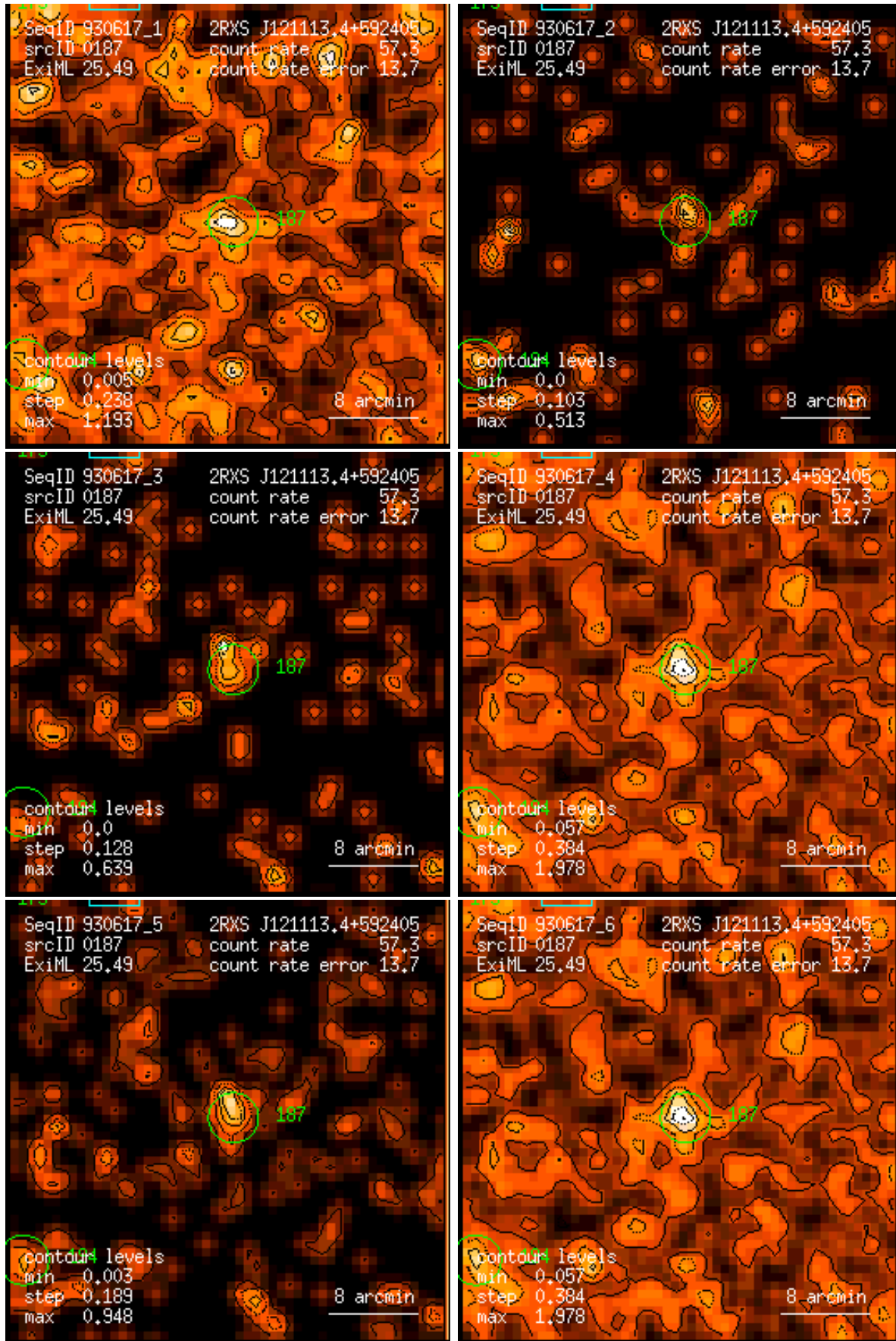
Figure 187: RASS 930617: detection 0187: band rate images, Gaussian filter: (1) PSPC channels 11 – 41, (2) 52 – 90, (3) 91 – 201, (4) 11 – 235, (5) 52 – 201, (6) 11 – 201. Broad band rates in counts/ks. Band rate contour levels in counts/ks/arcmin 2 .
