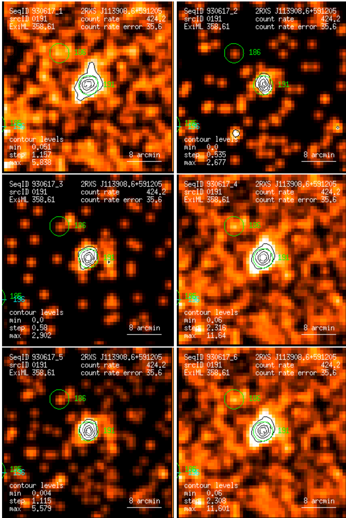
Figure 191: RASS 930617: detection 0191: band rate images, Gaussian filter: (1) PSPC channels 11 – 41, (2) 52 – 90, (3) 91 – 201, (4) 11 – 235, (5) 52 – 201, (6) 11 – 201. Broad band rates in counts/ks. Band rate contour levels in counts/ks/arcmin 2 .
