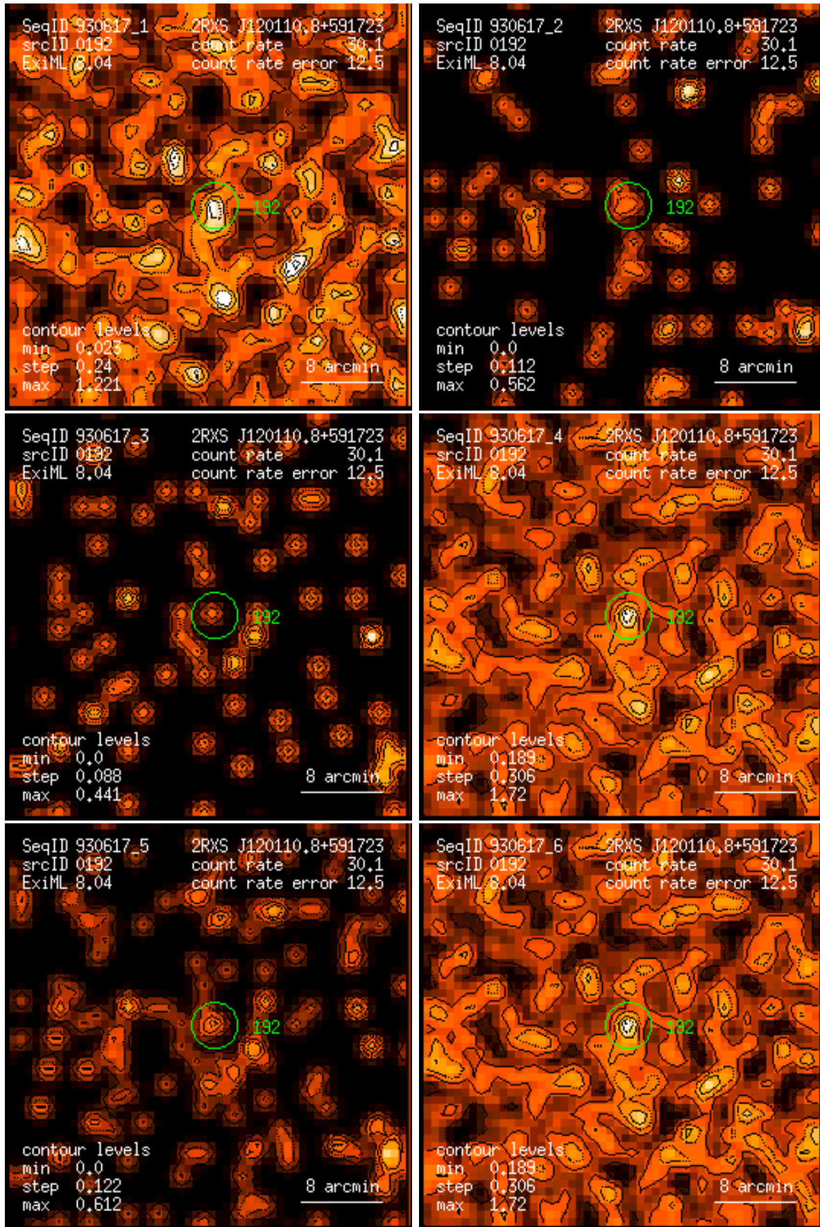
Figure 192: RASS 930617: detection 0192: band rate images, Gaussian filter: (1) PSPC channels 11 – 41, (2) 52 – 90, (3) 91 – 201, (4) 11 – 235, (5) 52 – 201, (6) 11 – 201. Broad band rates in counts/ks. Band rate contour levels in counts/ks/arcmin 2 .
