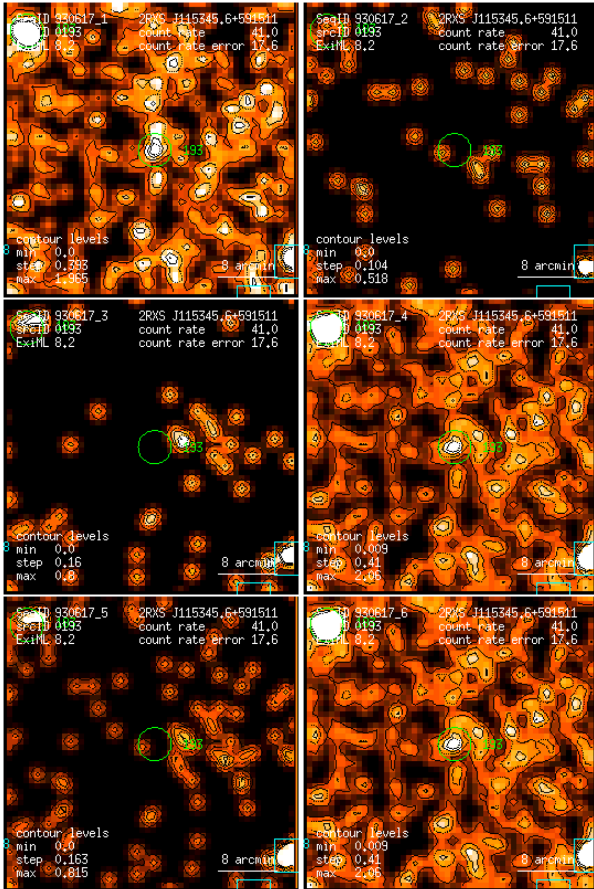
Figure 193: RASS 930617: detection 0193: band rate images, Gaussian filter: (1) PSPC channels 11 – 41, (2) 52 – 90, (3) 91 – 201, (4) 11 – 235, (5) 52 – 201, (6) 11 – 201. Broad band rates in counts/ks. Band rate contour levels in counts/ks/arcmin 2 .
