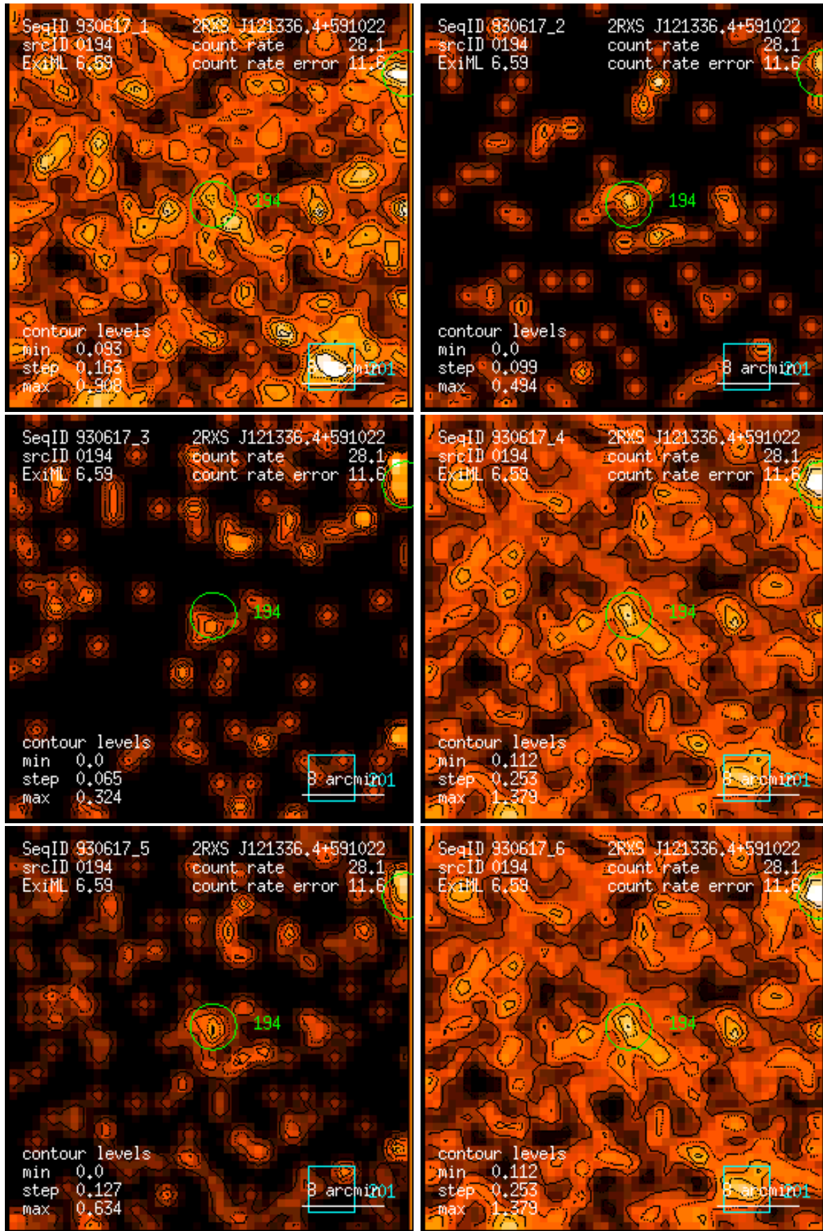
Figure 194: RASS 930617: detection 0194: band rate images, Gaussian filter: (1) PSPC channels 11 – 41, (2) 52 – 90, (3) 91 – 201, (4) 11 – 235, (5) 52 – 201, (6) 11 – 201. Broad band rates in counts/ks. Band rate contour levels in counts/ks/arcmin 2 .
