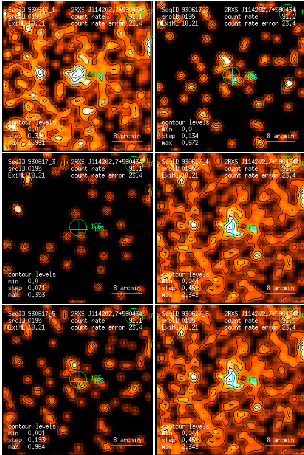
Figure 195: RASS 930617: detection 0195: band rate images, Gaussian filter: (1) PSPC channels 11 – 41, (2) 52 – 90, (3) 91 – 201, (4) 11 – 235, (5) 52 – 201, (6) 11 – 201. Broad band rates in counts/ks. Band rate contour levels in counts/ks/arcmin 2 .
