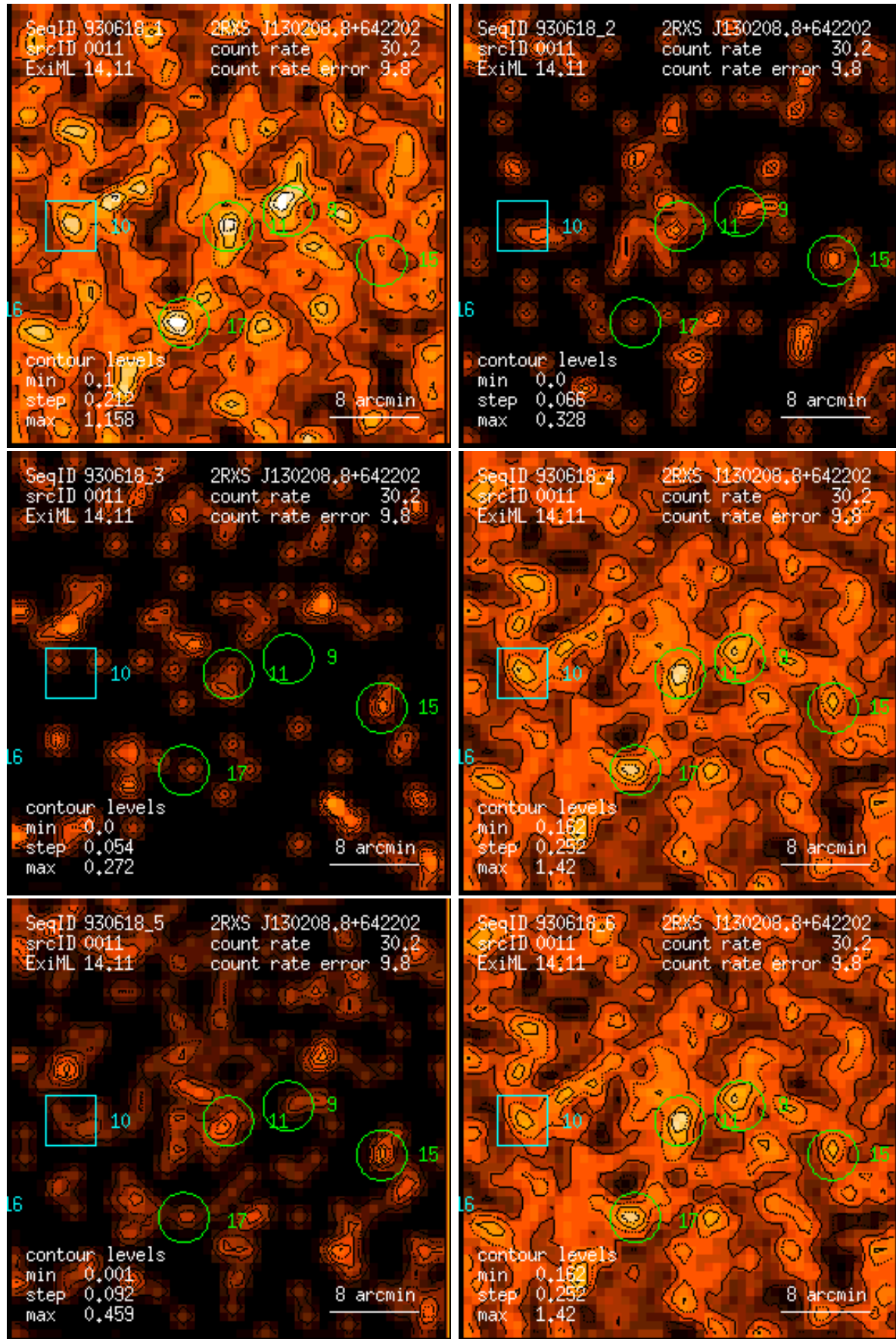
Figure 11: RASS 930618: detection 0011: band rate images, Gaussian filter: (1) PSPC channels 11 – 41, (2) 52 – 90, (3) 91 – 201, (4) 11 – 235, (5) 52 – 201, (6) 11 – 201. Broad band rates in counts/ks. Band rate contour levels in counts/ks/arcmin 2 .
