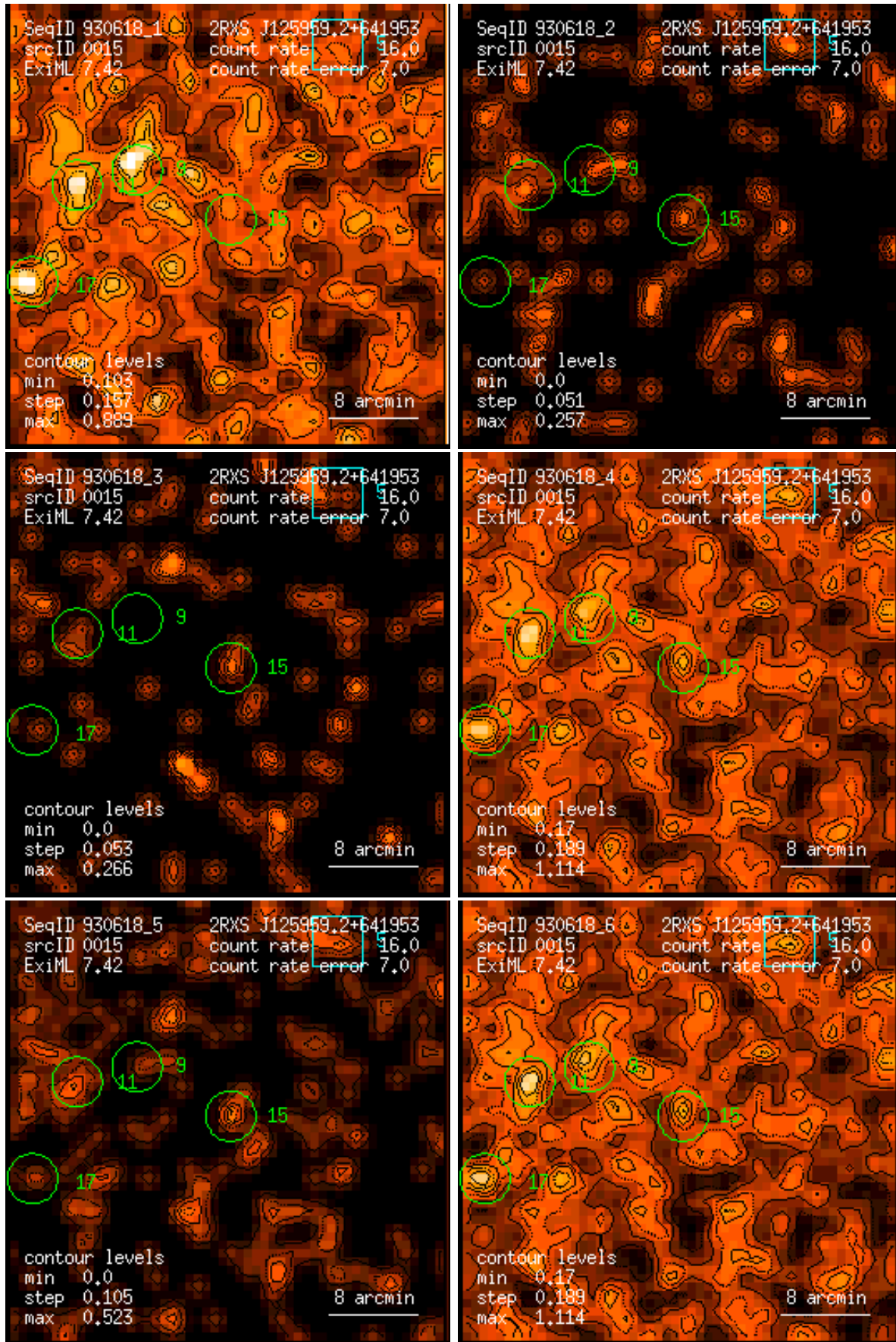
Figure 15: RASS 930618: detection 0015: band rate images, Gaussian filter: (1) PSPC channels 11 – 41, (2) 52 – 90, (3) 91 – 201, (4) 11 – 235, (5) 52 – 201, (6) 11 – 201. Broad band rates in counts/ks. Band rate contour levels in counts/ks/arcmin 2 .
