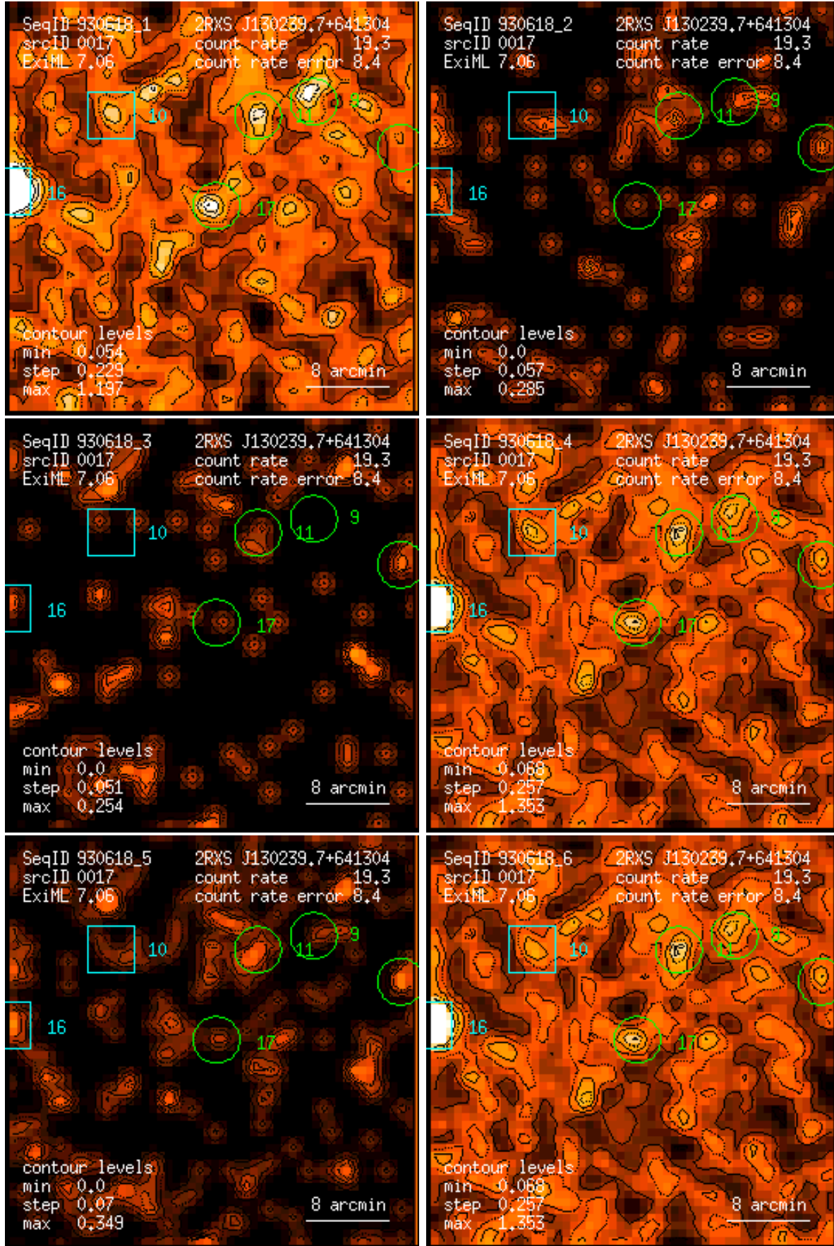
Figure 17: RASS 930618: detection 0017: band rate images, Gaussian filter: (1) PSPC channels 11 – 41, (2) 52 – 90, (3) 91 – 201, (4) 11 – 235, (5) 52 – 201, (6) 11 – 201. Broad band rates in counts/ks. Band rate contour levels in counts/ks/arcmin 2 .
