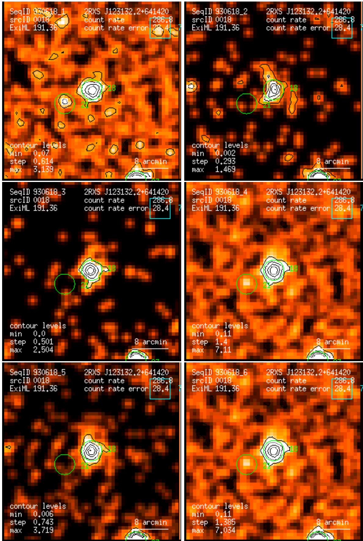
Figure 18: RASS 930618: detection 0018: band rate images, Gaussian filter: (1) PSPC channels 11 – 41, (2) 52 – 90, (3) 91 – 201, (4) 11 – 235, (5) 52 – 201, (6) 11 – 201. Broad band rates in counts/ks. Band rate contour levels in counts/ks/arcmin 2 .
