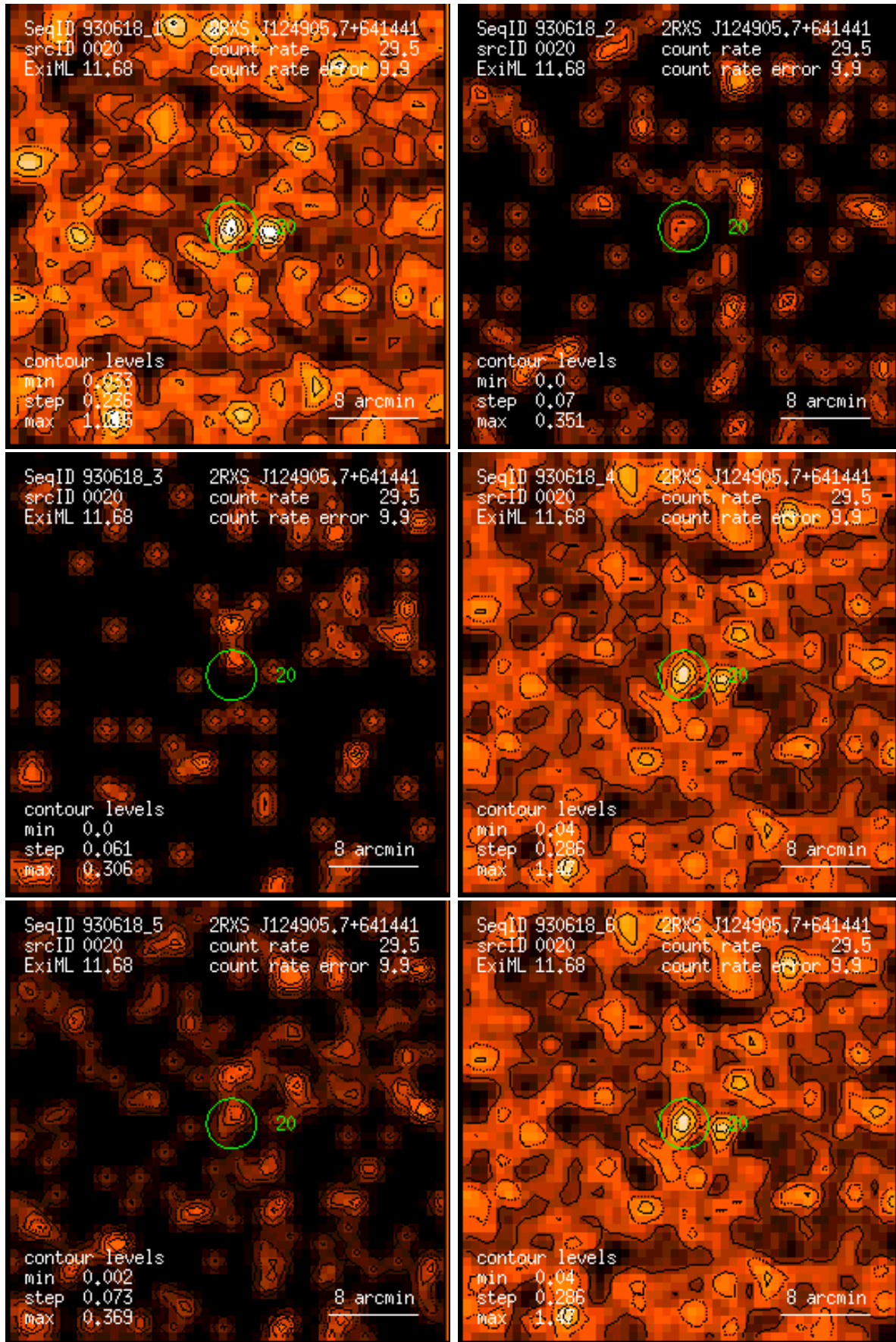
Figure 20: RASS 930618: detection 0020: band rate images, Gaussian filter: (1) PSPC channels 11 – 41, (2) 52 – 90, (3) 91 – 201, (4) 11 – 235, (5) 52 – 201, (6) 11 – 201. Broad band rates in counts/ks. Band rate contour levels in counts/ks/arcmin 2 .
