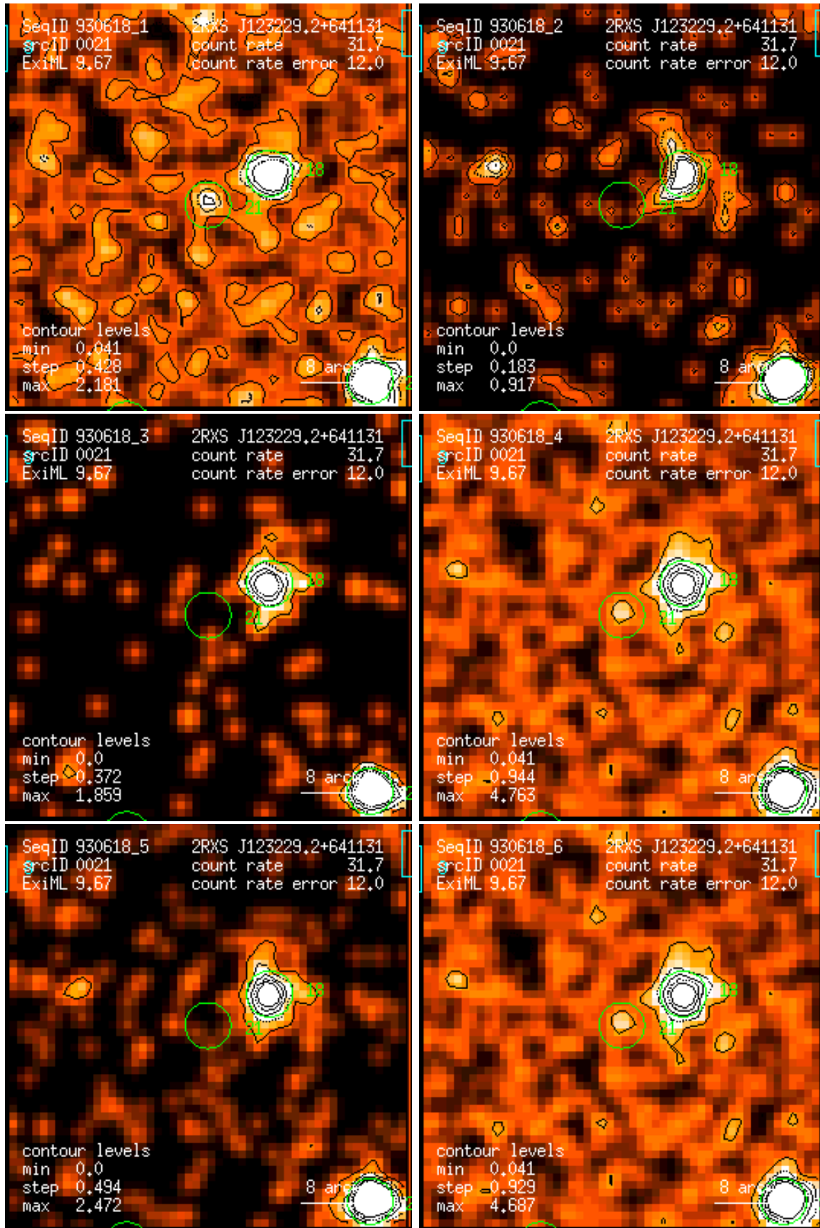
Figure 21: RASS 930618: detection 0021: band rate images, Gaussian filter: (1) PSPC channels 11 – 41, (2) 52 – 90, (3) 91 – 201, (4) 11 – 235, (5) 52 – 201, (6) 11 – 201. Broad band rates in counts/ks. Band rate contour levels in counts/ks/arcmin 2 .
