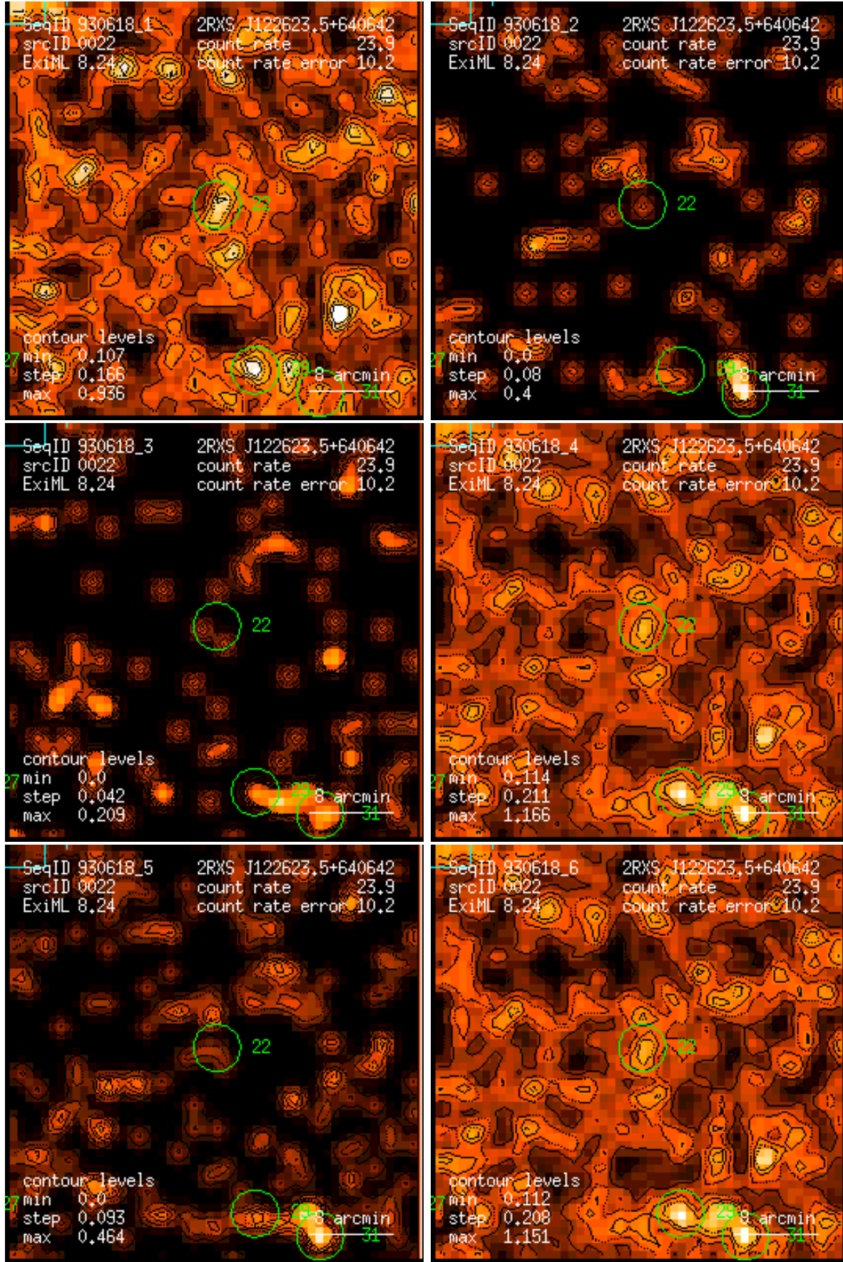
Figure 22: RASS 930618: detection 0022: band rate images, Gaussian filter: (1) PSPC channels 11 – 41, (2) 52 – 90, (3) 91 – 201, (4) 11 – 235, (5) 52 – 201, (6) 11 – 201. Broad band rates in counts/ks. Band rate contour levels in counts/ks/arcmin 2 .
