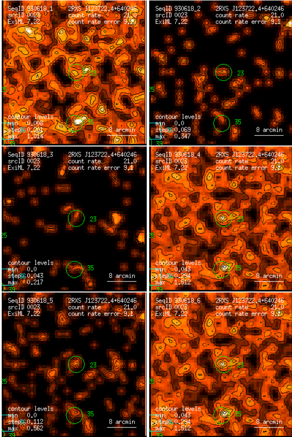
Figure 23: RASS 930618: detection 0023: band rate images, Gaussian filter: (1) PSPC channels 11 – 41, (2) 52 – 90, (3) 91 – 201, (4) 11 – 235, (5) 52 – 201, (6) 11 – 201. Broad band rates in counts/ks. Band rate contour levels in counts/ks/arcmin 2 .
