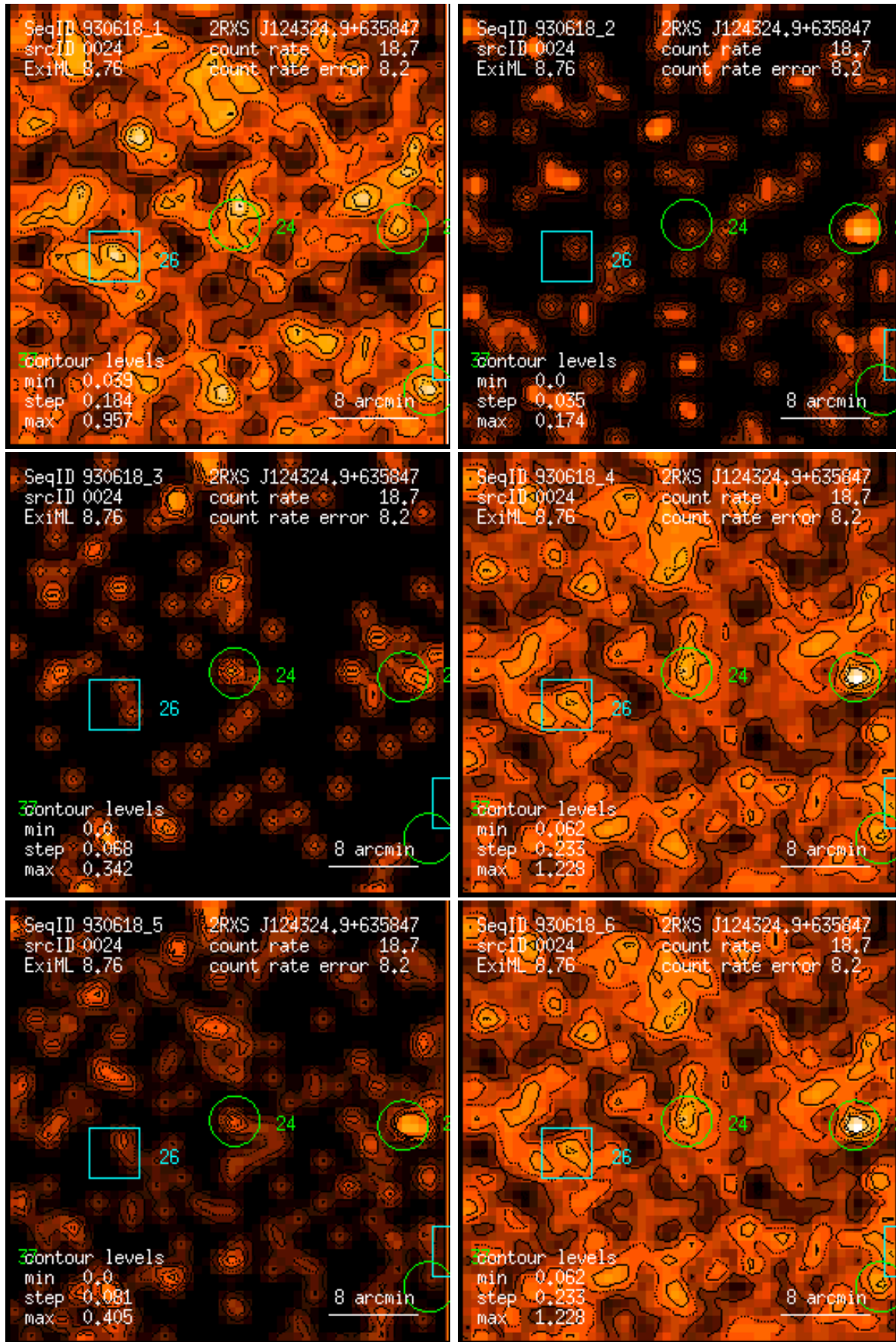
Figure 24: RASS 930618: detection 0024: band rate images, Gaussian filter: (1) PSPC channels 11 – 41, (2) 52 – 90, (3) 91 – 201, (4) 11 – 235, (5) 52 – 201, (6) 11 – 201. Broad band rates in counts/ks. Band rate contour levels in counts/ks/arcmin 2 .
